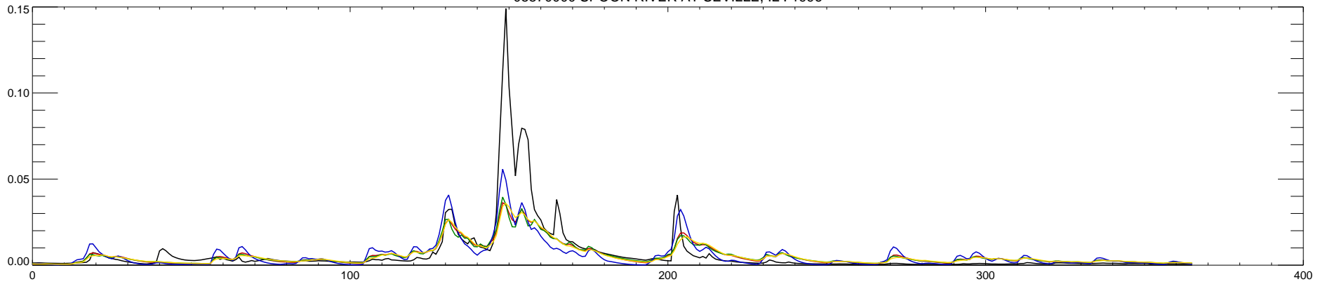
05570000 SPOON RIVER AT SEVILLE, IL : 1997
