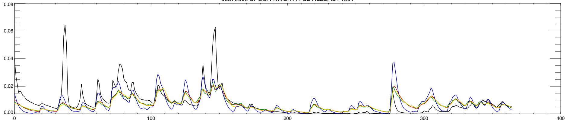
05570000 SPOON RIVER AT SEVILLE, IL : 1992
