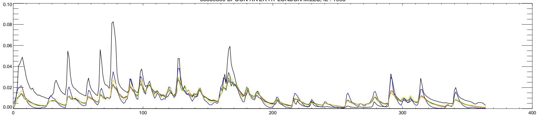
05569500 SPOON RIVER AT LONDON MILLS, IL : 1998
