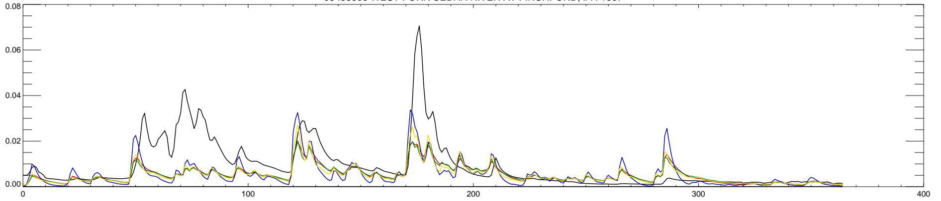
05458900 WEST FORK CEDAR RIVER AT FINCHFORD, IA : 1998
