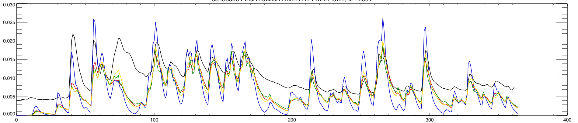
05435500 PECATONICA RIVER AT FREEPORT, IL : 2001
