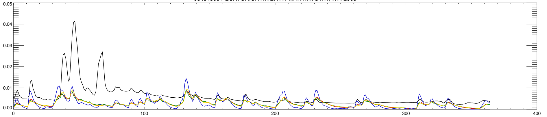
05434500 PECATONICA RIVER AT MARTINTOWN, WI : 2006
