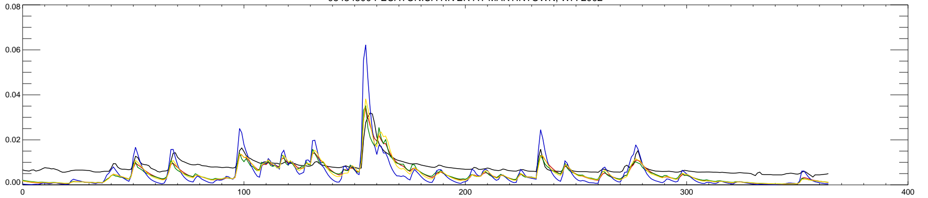
05434500 PECATONICA RIVER AT MARTINTOWN, WI : 2003
