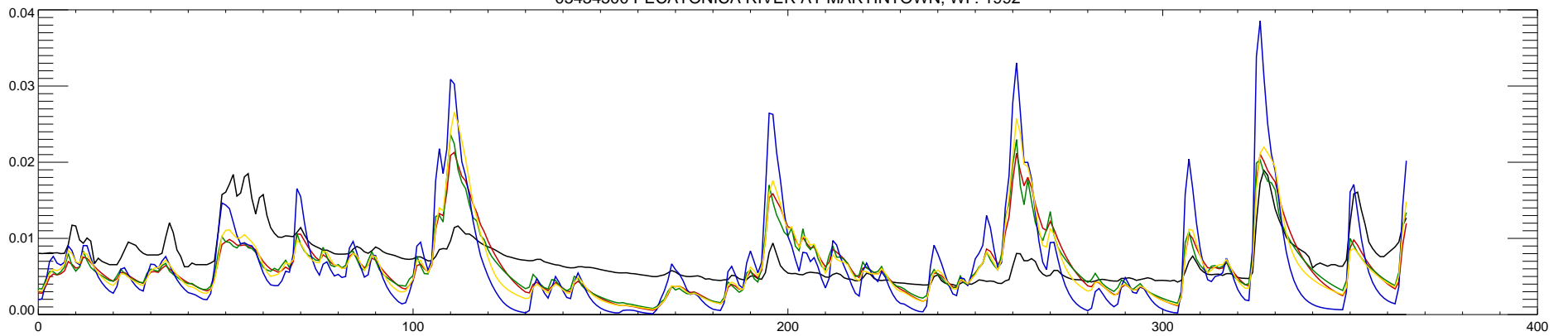
05434500 PECATONICA RIVER AT MARTINTOWN, WI : 1992
