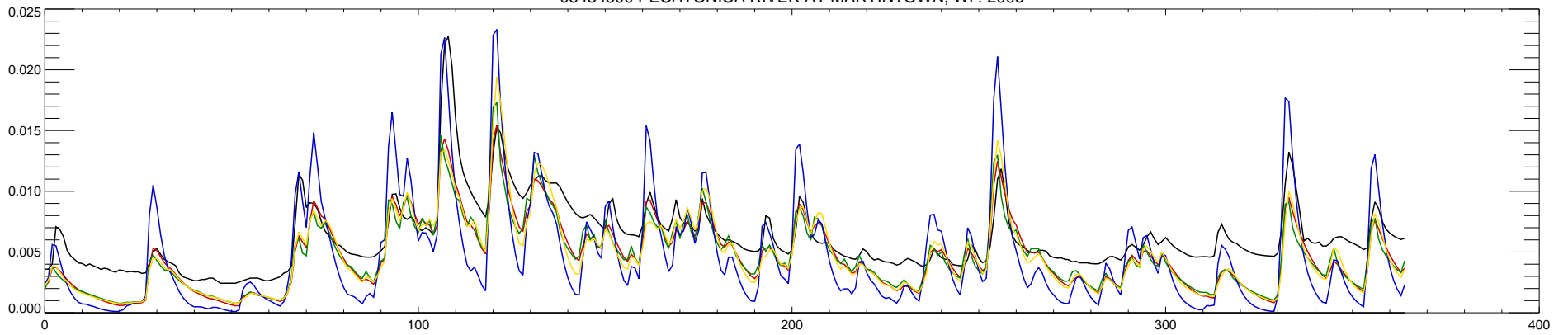
05434500 PECATONICA RIVER AT MARTINTOWN, WI : 2007
