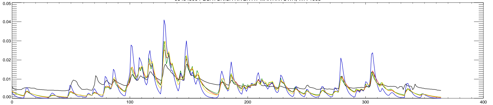
05434500 PECATONICA RIVER AT MARTINTOWN, WI : 1995
