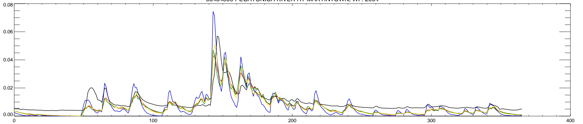
05434500 PECATONICA RIVER AT MARTINTOWN, WI : 2004
