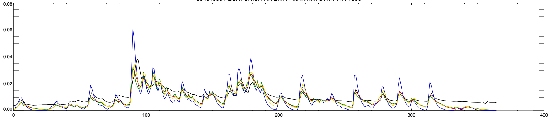
05434500 PECATONICA RIVER AT MARTINTOWN, WI : 1998
