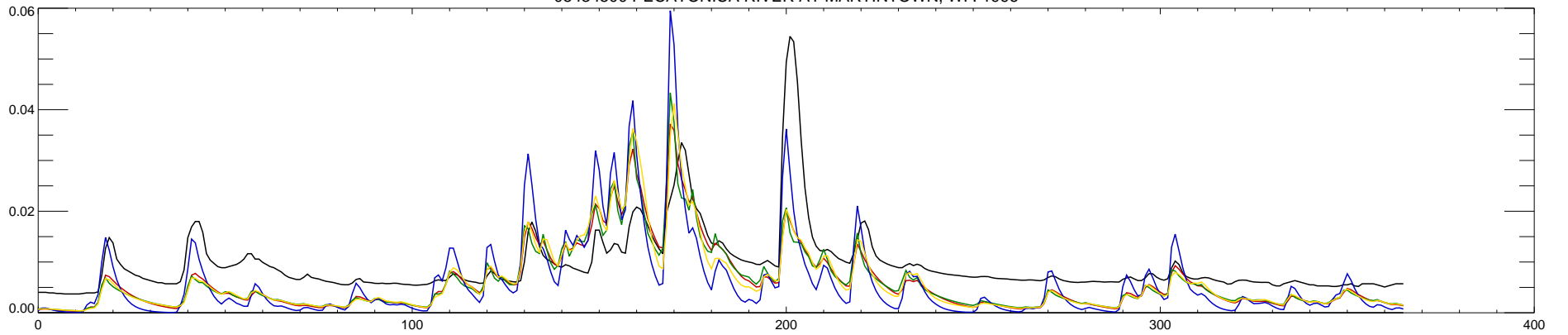
05434500 PECATONICA RIVER AT MARTINTOWN, WI : 1997
