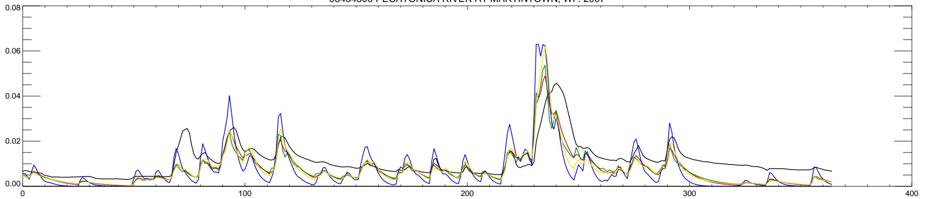
05434500 PECATONICA RIVER AT MARTINTOWN, WI : 2007
