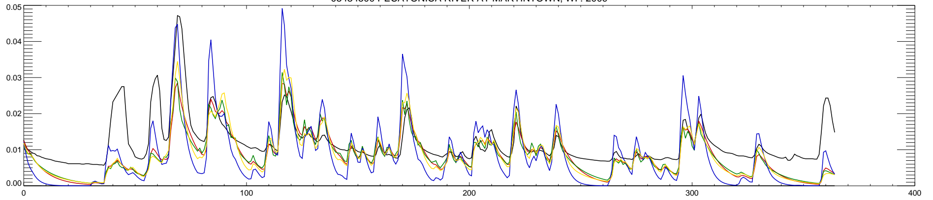
05434500 PECATONICA RIVER AT MARTINTOWN, WI : 2009
