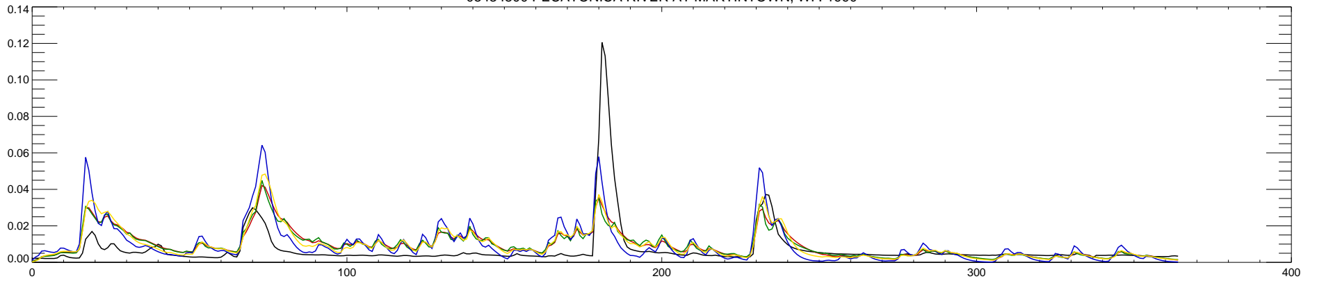
05434500 PECATONICA RIVER AT MARTINTOWN, WI : 1991
