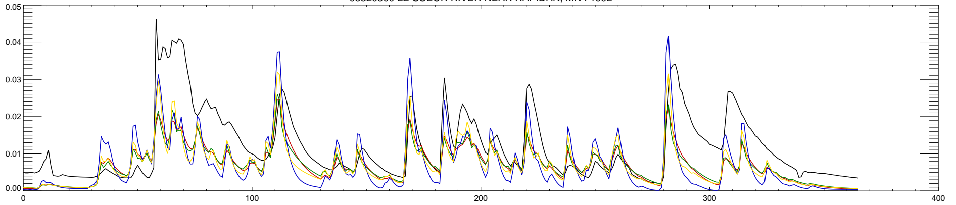
05320500 LE SUEUR RIVER NEAR RAPIDAN, MN : 1992
