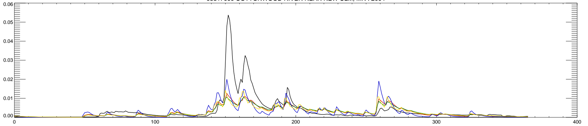
05317000 COTTONWOOD RIVER NEAR NEW ULM, MN : 2004
