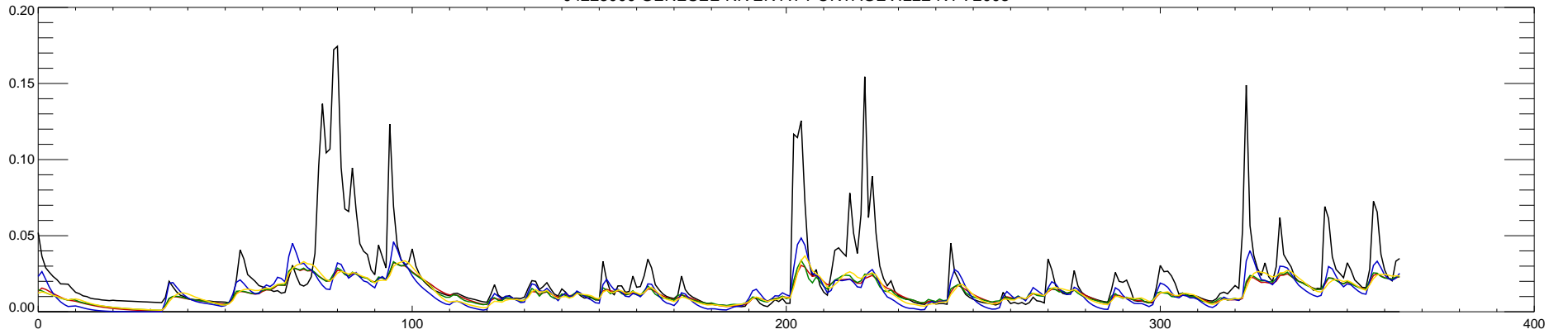
04223000 GENESEE RIVER AT PORTAGEVILLE NY : 2004
