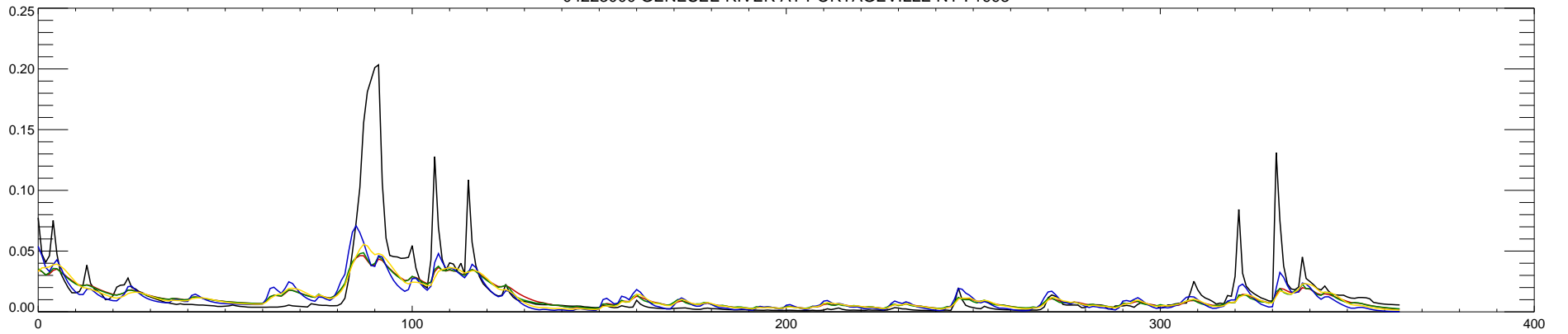
04223000 GENESEE RIVER AT PORTAGEVILLE NY : 1994
