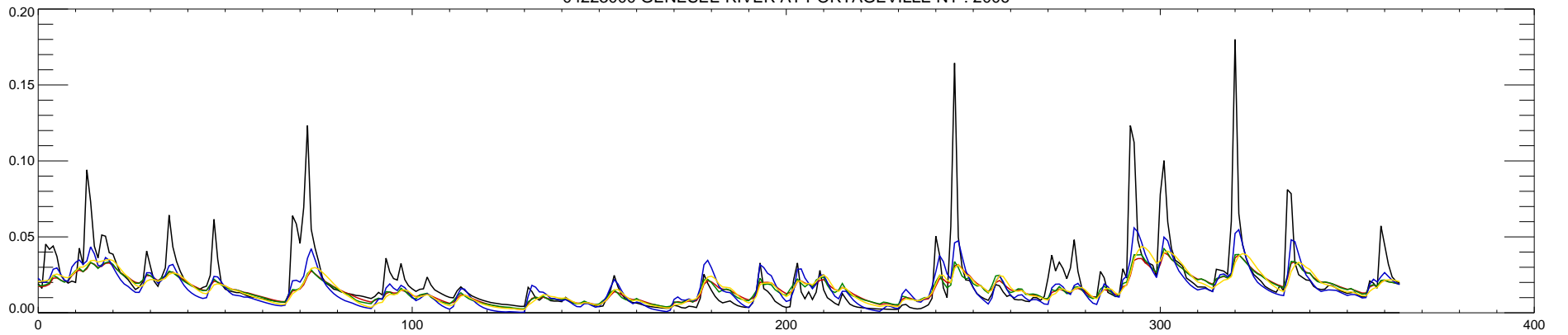
04223000 GENESEE RIVER AT PORTAGEVILLE NY : 2007
