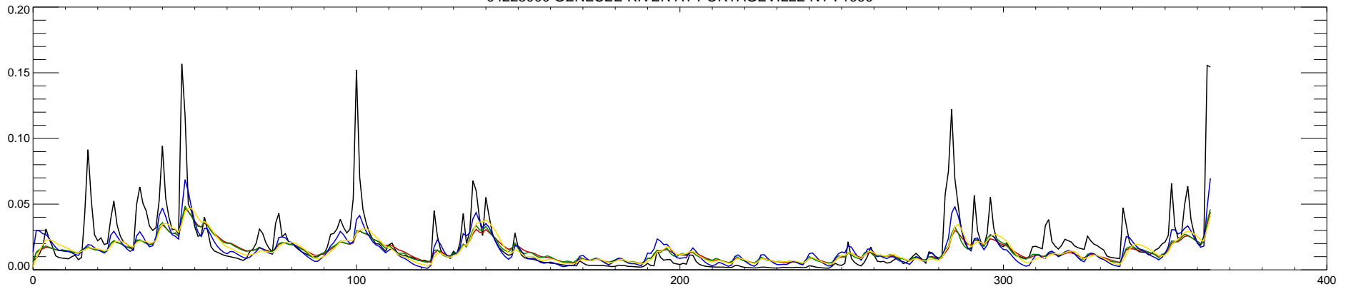
04223000 GENESEE RIVER AT PORTAGEVILLE NY : 1991
