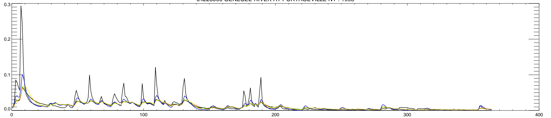
04223000 GENESEE RIVER AT PORTAGEVILLE NY : 1998
