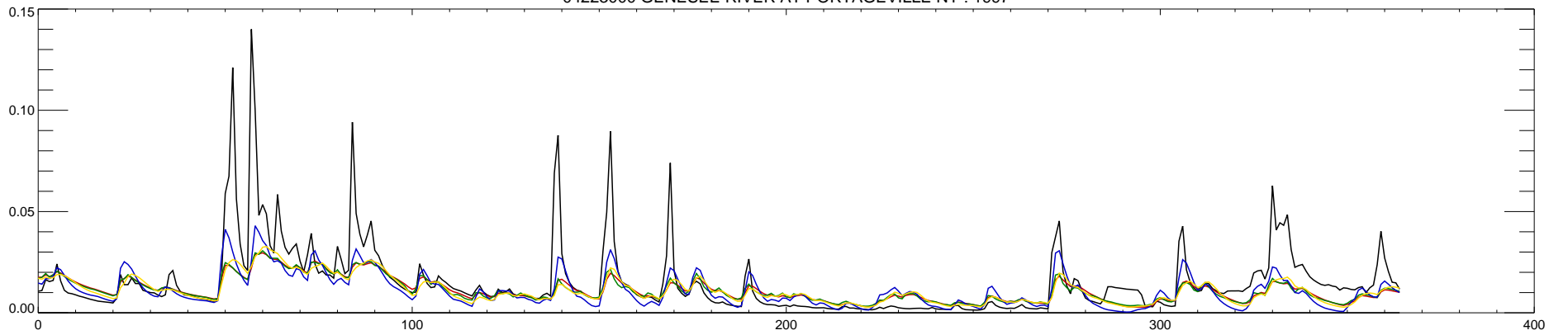
04223000 GENESEE RIVER AT PORTAGEVILLE NY : 1998
