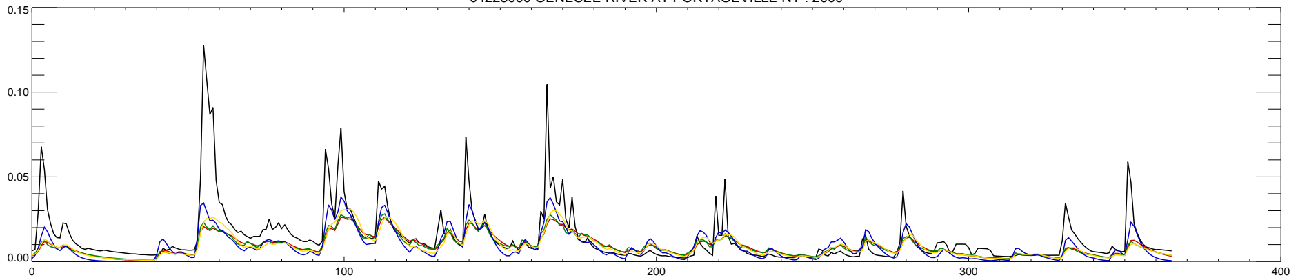
04223000 GENESEE RIVER AT PORTAGEVILLE NY : 2001
