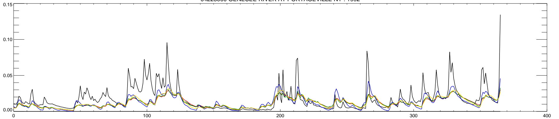
04223000 GENESEE RIVER AT PORTAGEVILLE NY : 1992
