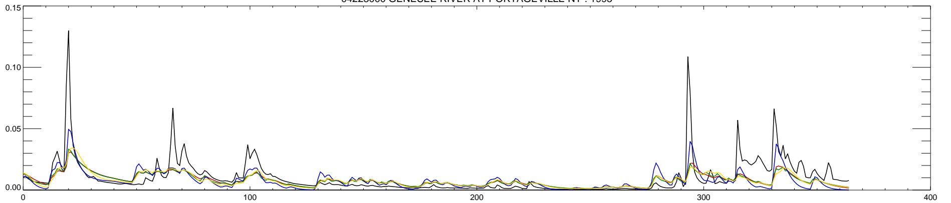
04223000 GENESEE RIVER AT PORTAGEVILLE NY : 1995
