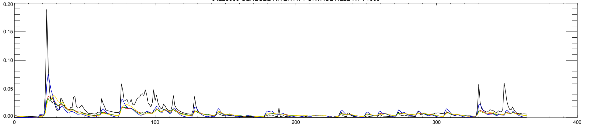
04223000 GENESEE RIVER AT PORTAGEVILLE NY : 2000
