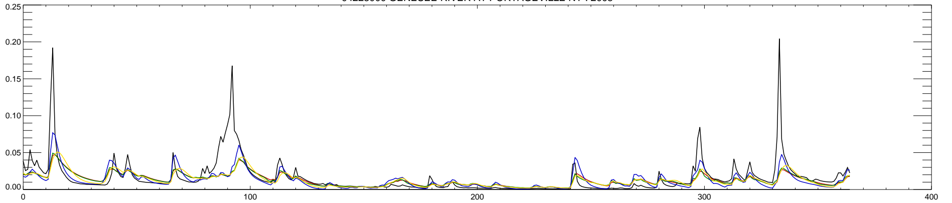
04223000 GENESEE RIVER AT PORTAGEVILLE NY : 2006
