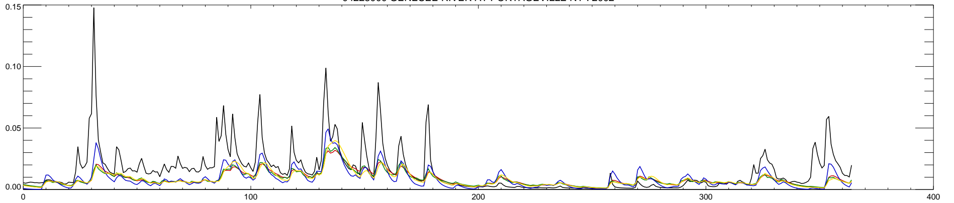
04223000 GENESEE RIVER AT PORTAGEVILLE NY : 2003
