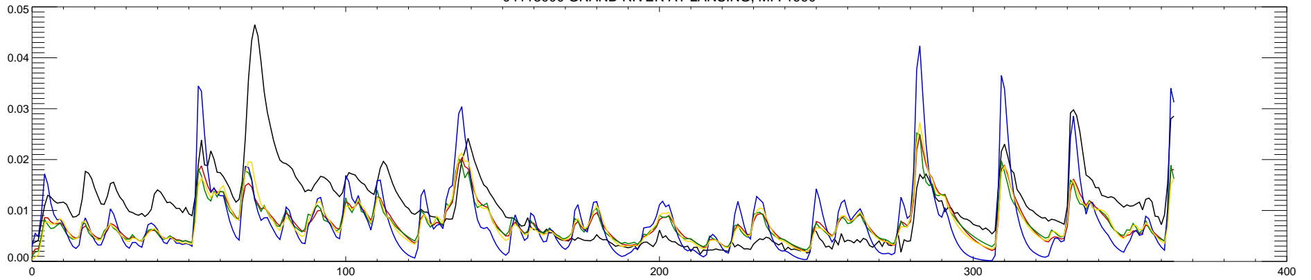
04113000 GRAND RIVER AT LANSING, MI : 1991
