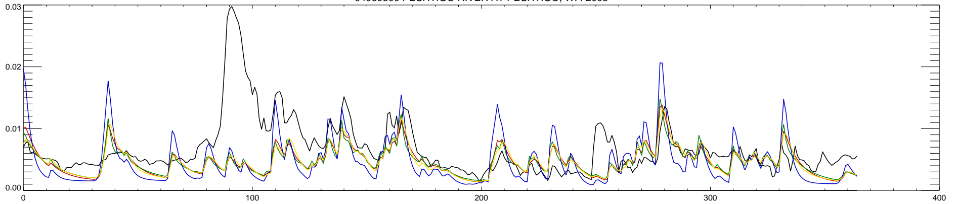
04069500 PESHTIGO RIVER AT PESHTIGO, WI : 2006
