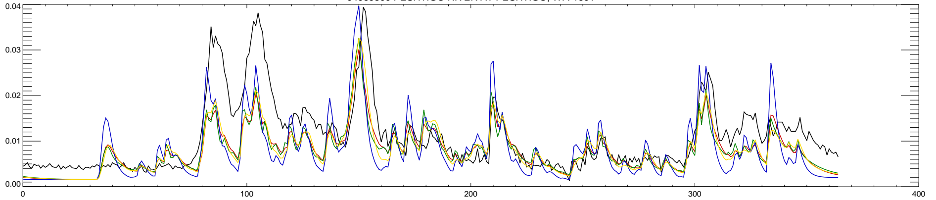
04069500 PESHTIGO RIVER AT PESHTIGO, WI : 1992
