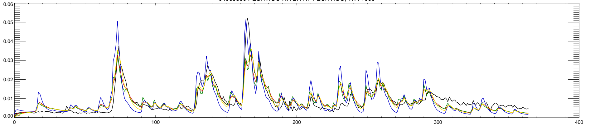
04069500 PESHTIGO RIVER AT PESHTIGO, WI : 1991
