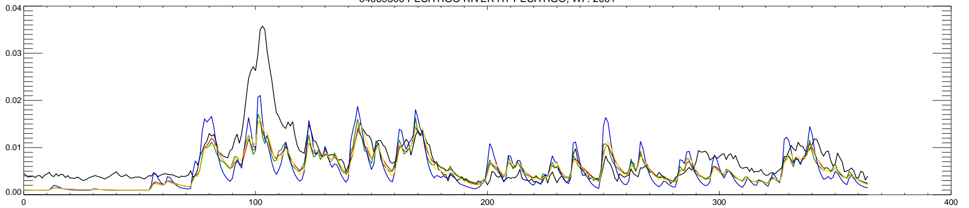
04069500 PESHTIGO RIVER AT PESHTIGO, WI : 2001
