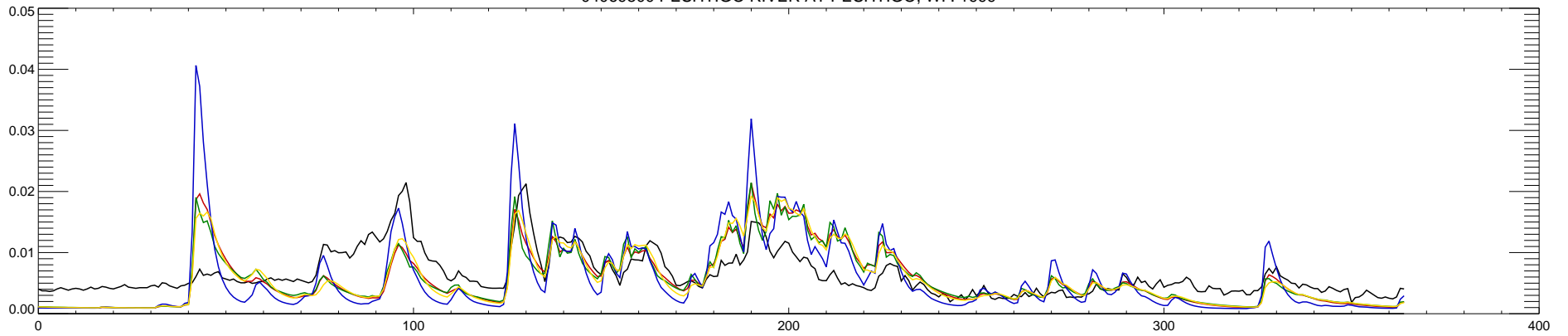
04069500 PESHTIGO RIVER AT PESHTIGO, WI : 2000
