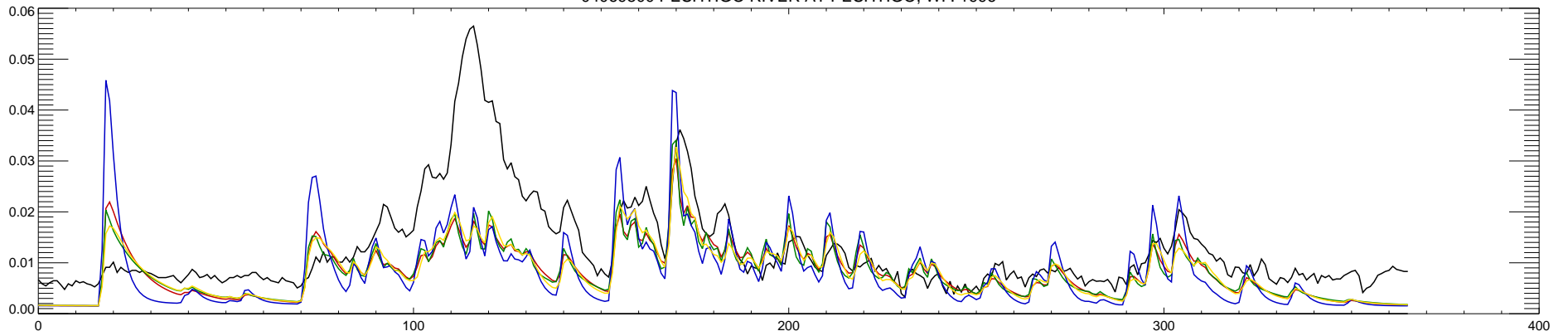
04069500 PESHTIGO RIVER AT PESHTIGO, WI : 1997
