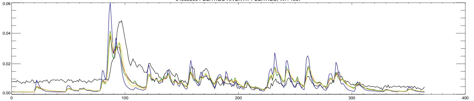
04069500 PESHTIGO RIVER AT PESHTIGO, WI : 1998
