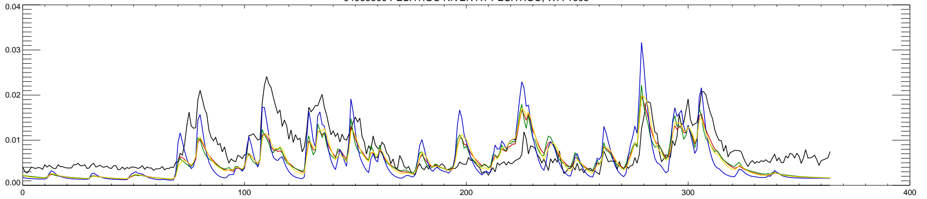
04069500 PESHTIGO RIVER AT PESHTIGO, WI : 1995
