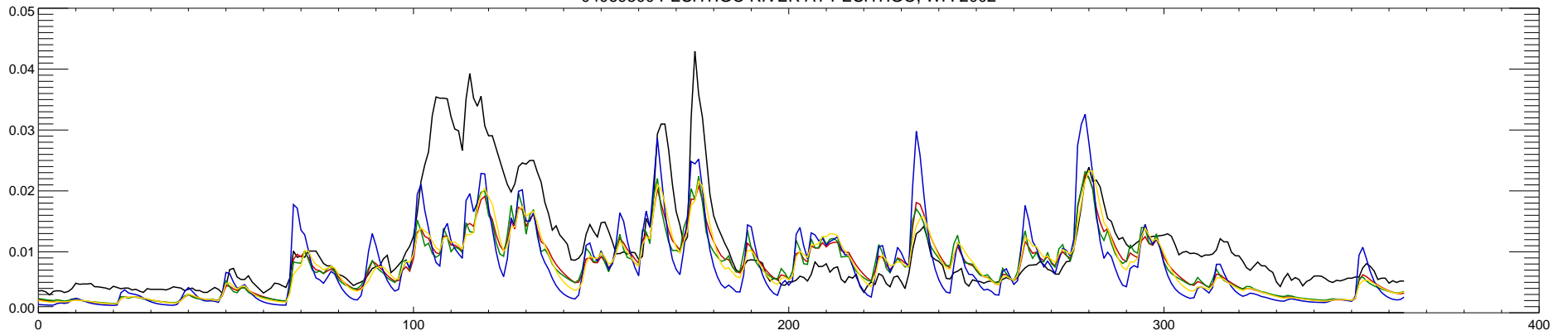
04069500 PESHTIGO RIVER AT PESHTIGO, WI : 2003
