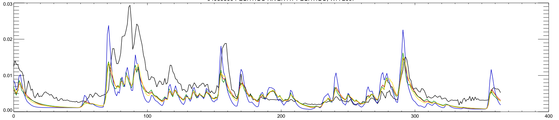
04069500 PESHTIGO RIVER AT PESHTIGO, WI : 2007
