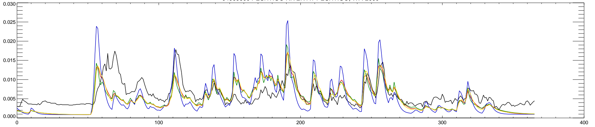
04069500 PESHTIGO RIVER AT PESHTIGO, WI : 2001
