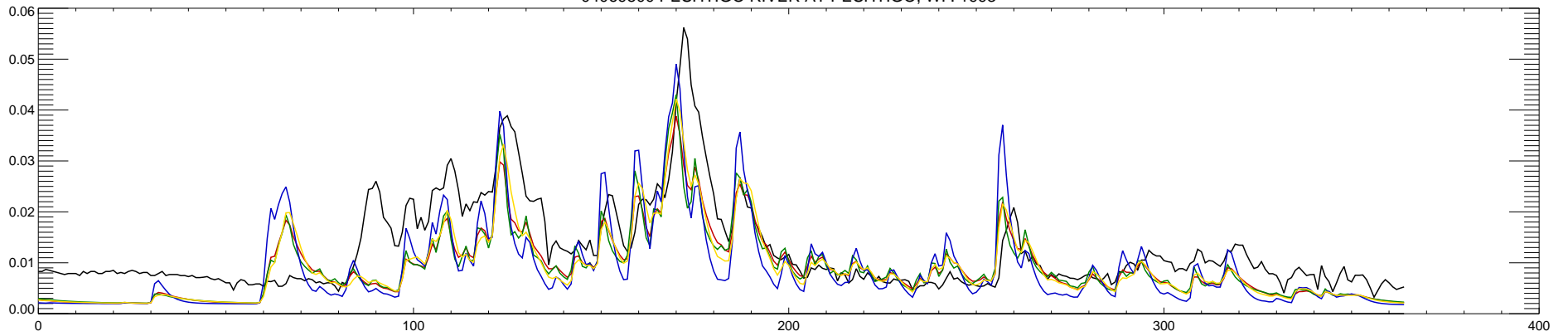
04069500 PESHTIGO RIVER AT PESHTIGO, WI : 1994
