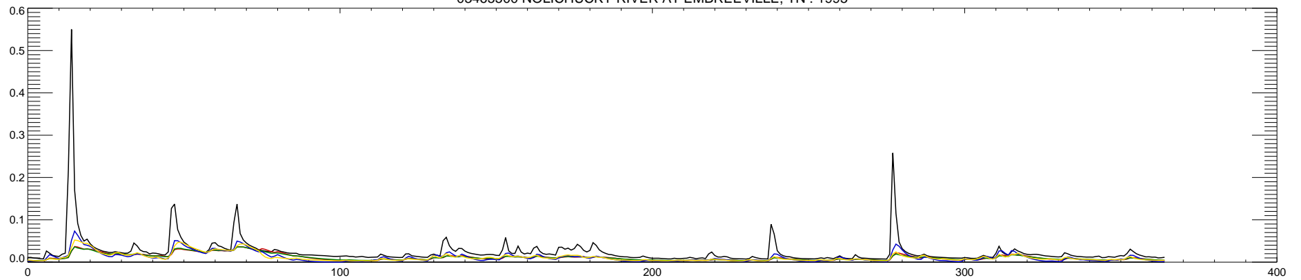
03465500 NOLICHUCKY RIVER AT EMBREEVILLE, TN : 1995
