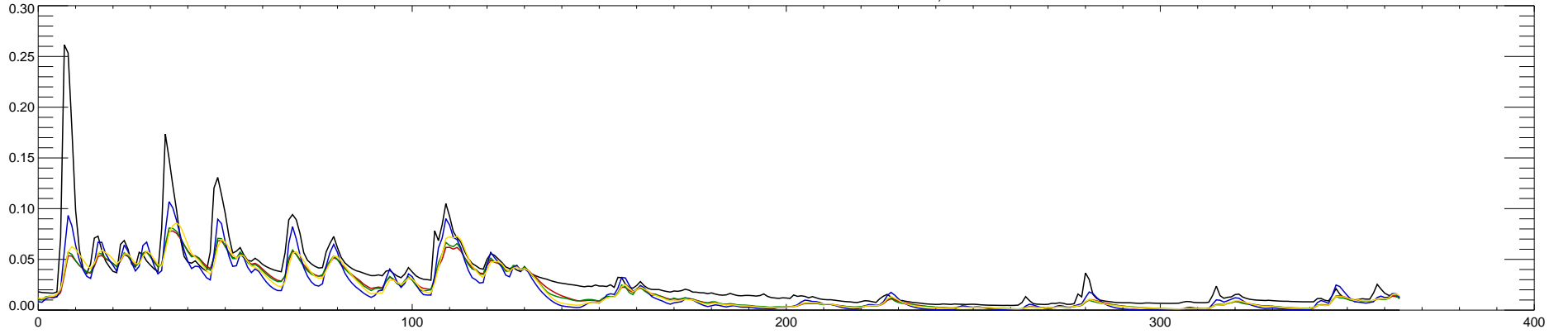
03451500 FRENCH BROAD RIVER AT ASHEVILLE, NC : 1998
