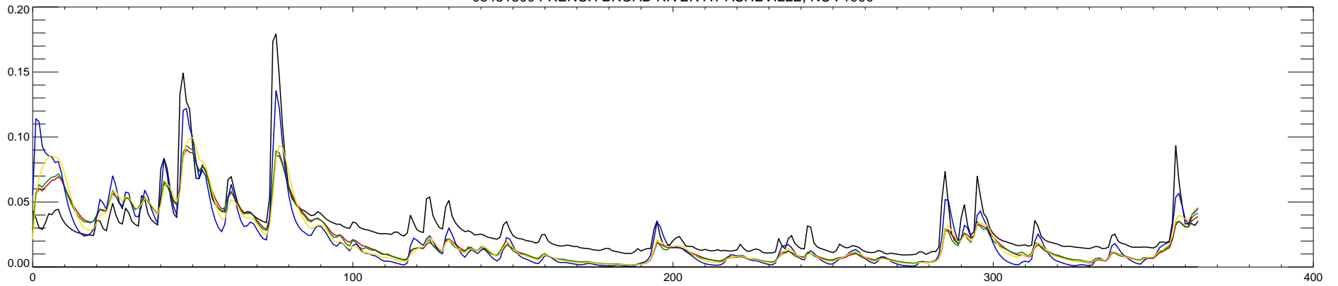
03451500 FRENCH BROAD RIVER AT ASHEVILLE, NC : 1991
