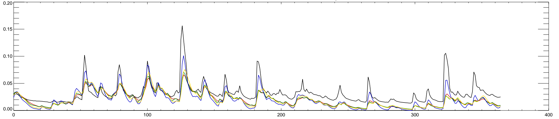
03451500 FRENCH BROAD RIVER AT ASHEVILLE, NC : 2004
