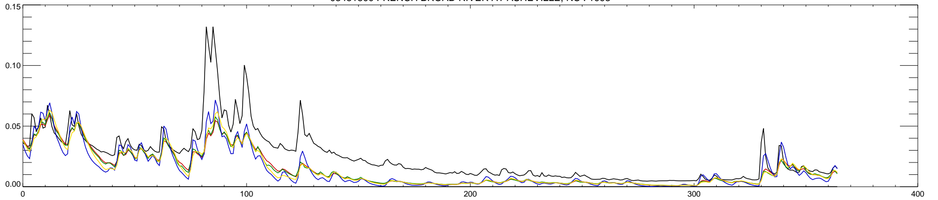
03451500 FRENCH BROAD RIVER AT ASHEVILLE, NC : 1994
