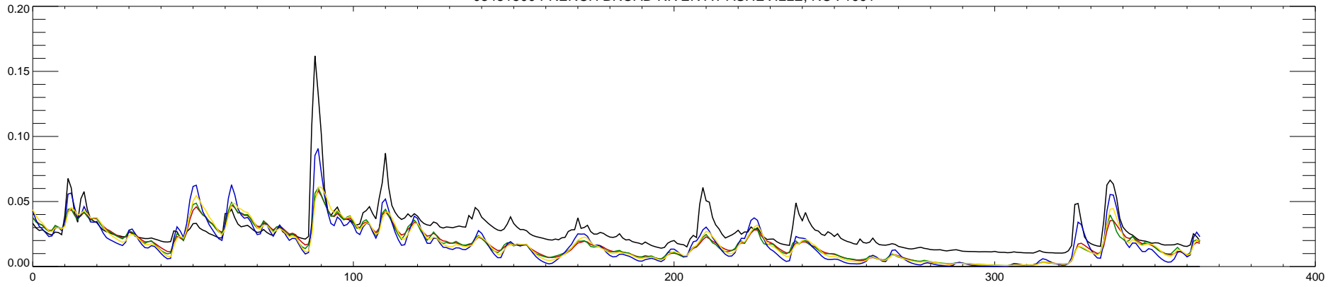
03451500 FRENCH BROAD RIVER AT ASHEVILLE, NC : 1992
