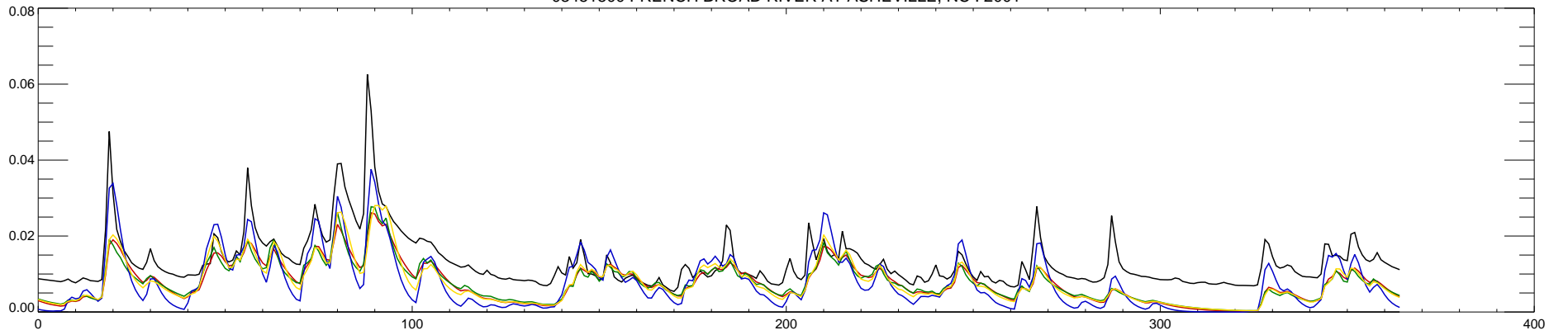
03451500 FRENCH BROAD RIVER AT ASHEVILLE, NC : 2001
