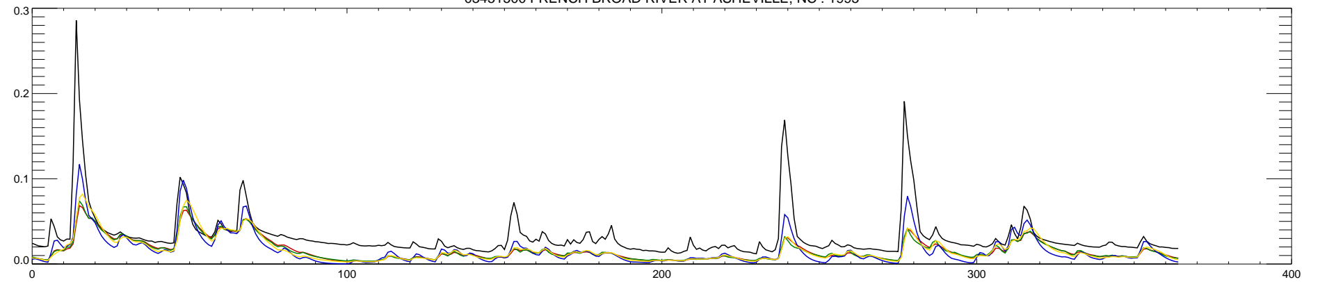
03451500 FRENCH BROAD RIVER AT ASHEVILLE, NC : 1995
