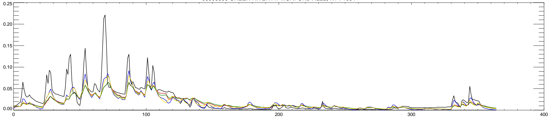
03308500 GREEN RIVER AT MUNFORDVILLE, KY : 1995
