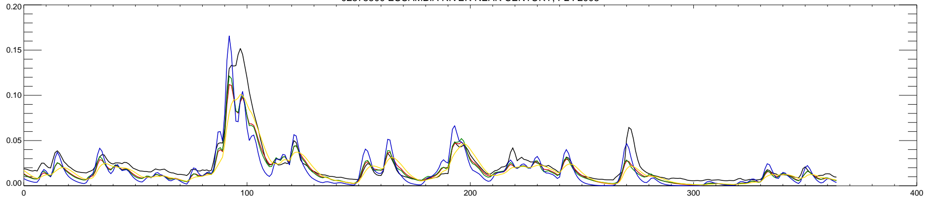
02375500 ESCAMBIA RIVER NEAR CENTURY, FL : 2006
