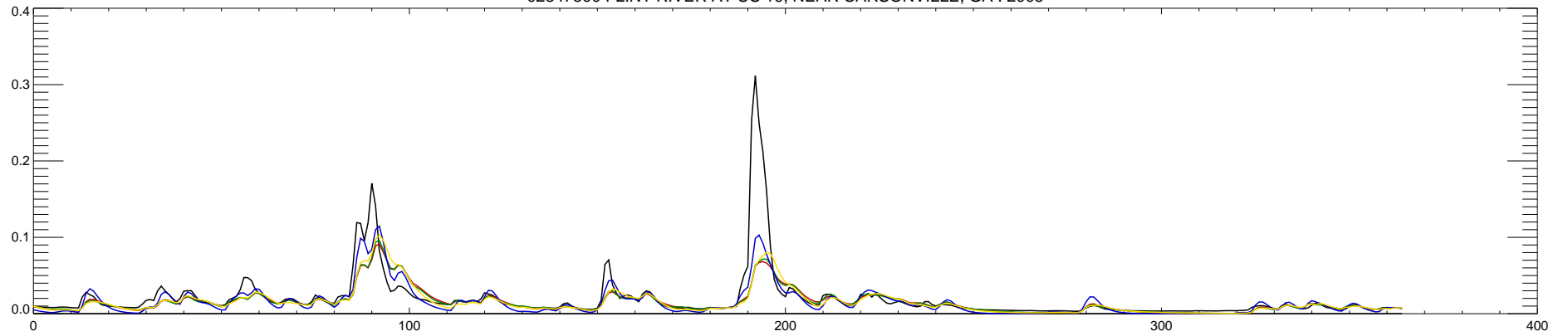
02347500 FLINT RIVER AT US 19, NEAR CARSONVILLE, GA : 2006
