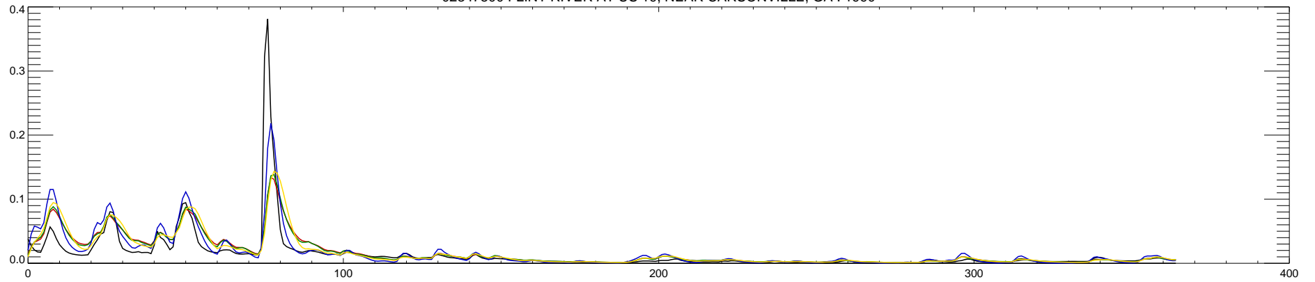
02347500 FLINT RIVER AT US 19, NEAR CARSONVILLE, GA : 1991
