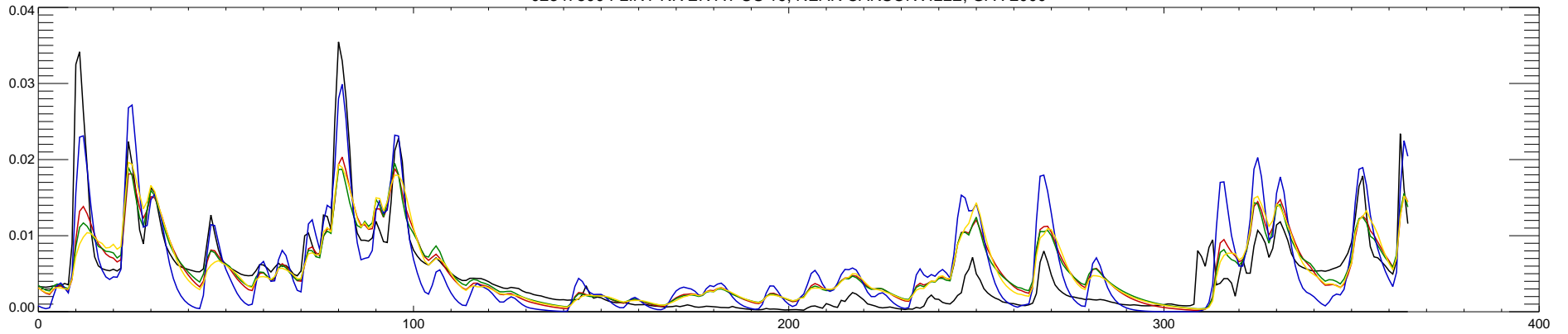
02347500 FLINT RIVER AT US 19, NEAR CARSONVILLE, GA : 2001
