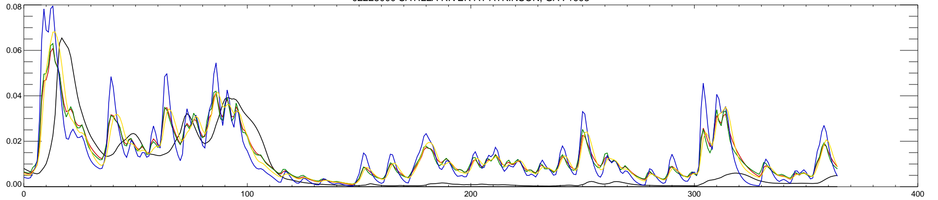
02228000 SATILLA RIVER AT ATKINSON, GA : 1994
