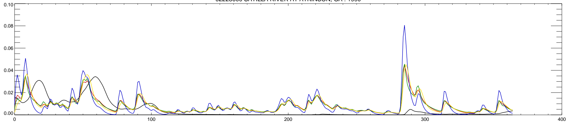
02228000 SATILLA RIVER AT ATKINSON, GA : 1991
