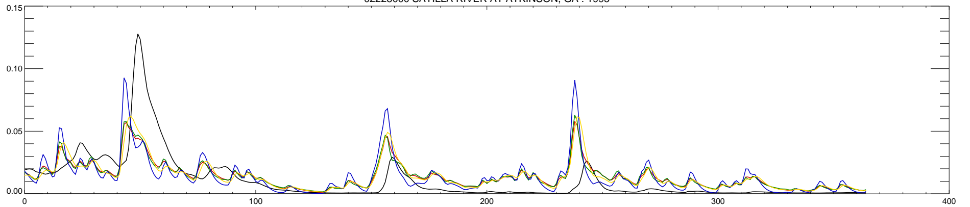
02228000 SATILLA RIVER AT ATKINSON, GA : 1995
