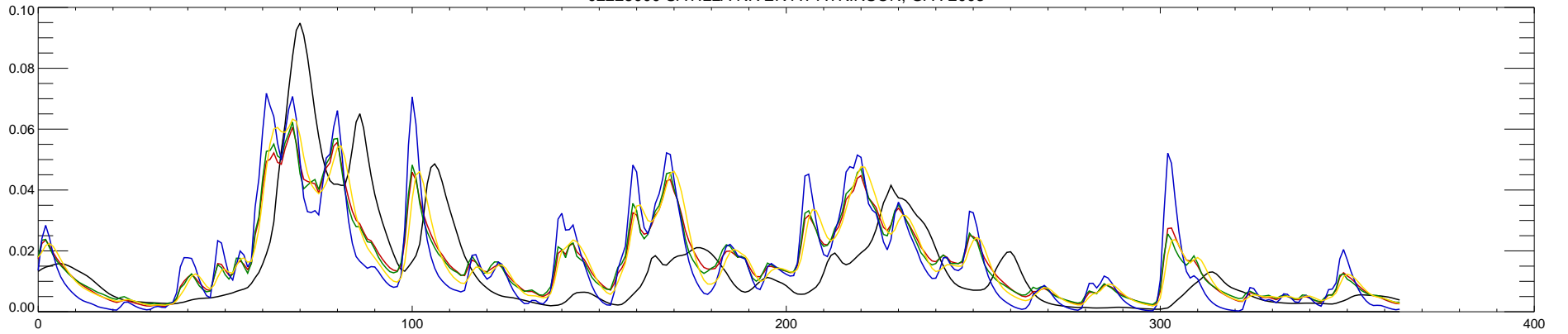
02228000 SATILLA RIVER AT ATKINSON, GA : 2004
