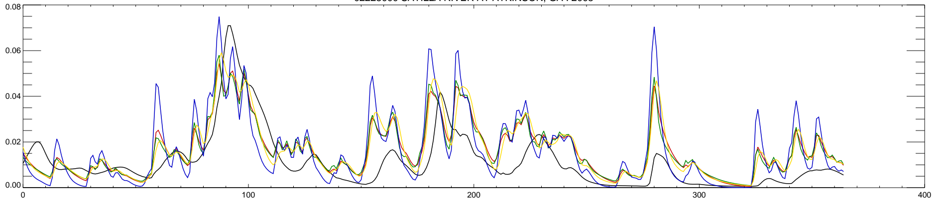
02228000 SATILLA RIVER AT ATKINSON, GA : 2006
