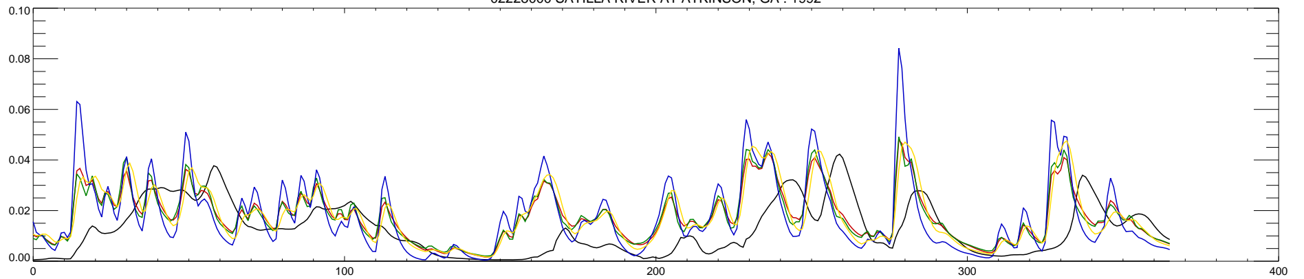
02228000 SATILLA RIVER AT ATKINSON, GA : 1992
