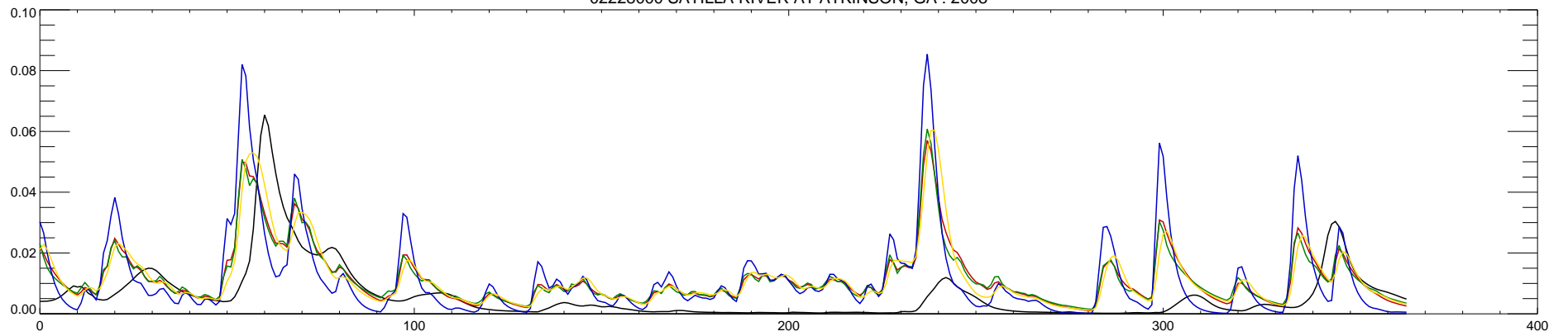
02228000 SATILLA RIVER AT ATKINSON, GA : 2009
