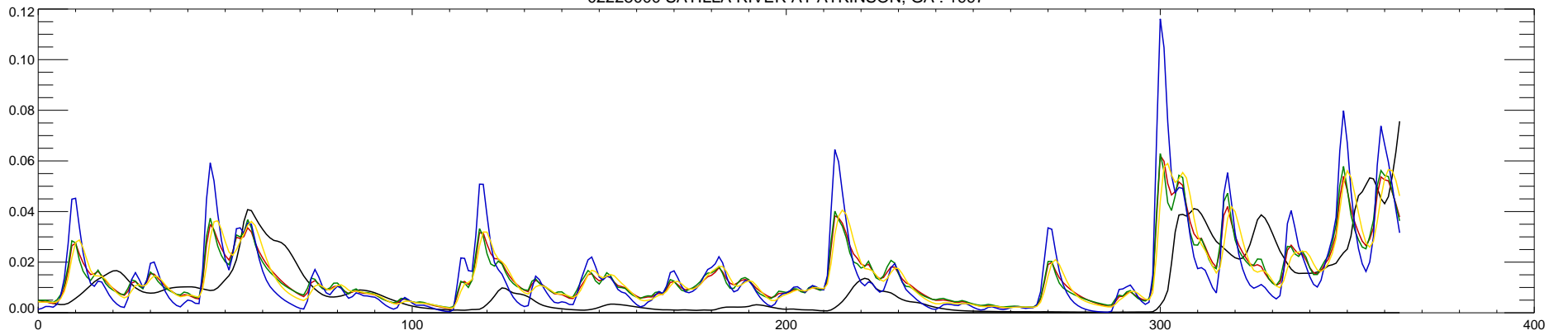
02228000 SATILLA RIVER AT ATKINSON, GA : 1998
