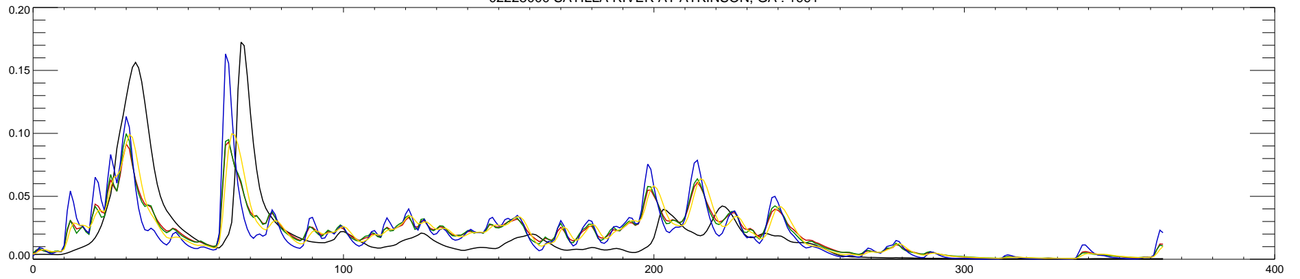
02228000 SATILLA RIVER AT ATKINSON, GA : 1992
