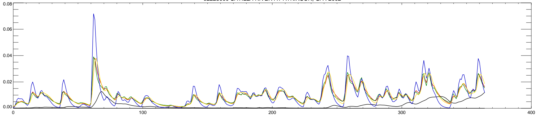
02228000 SATILLA RIVER AT ATKINSON, GA : 2003
