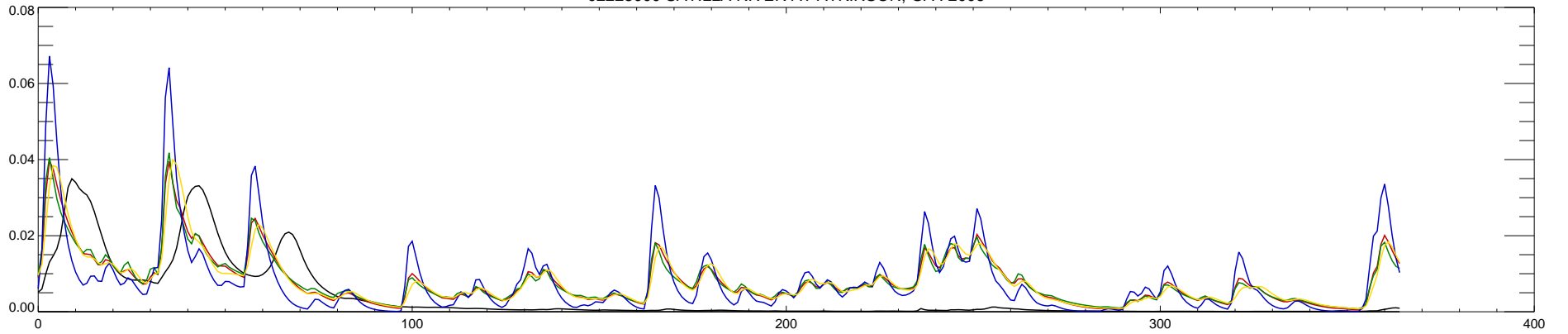
02228000 SATILLA RIVER AT ATKINSON, GA : 2007
