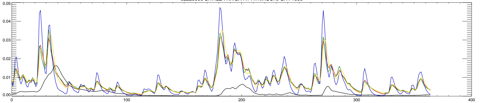
02228000 SATILLA RIVER AT ATKINSON, GA : 2000
