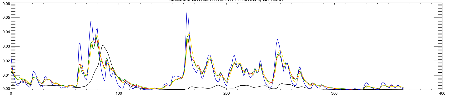
02228000 SATILLA RIVER AT ATKINSON, GA : 2001
