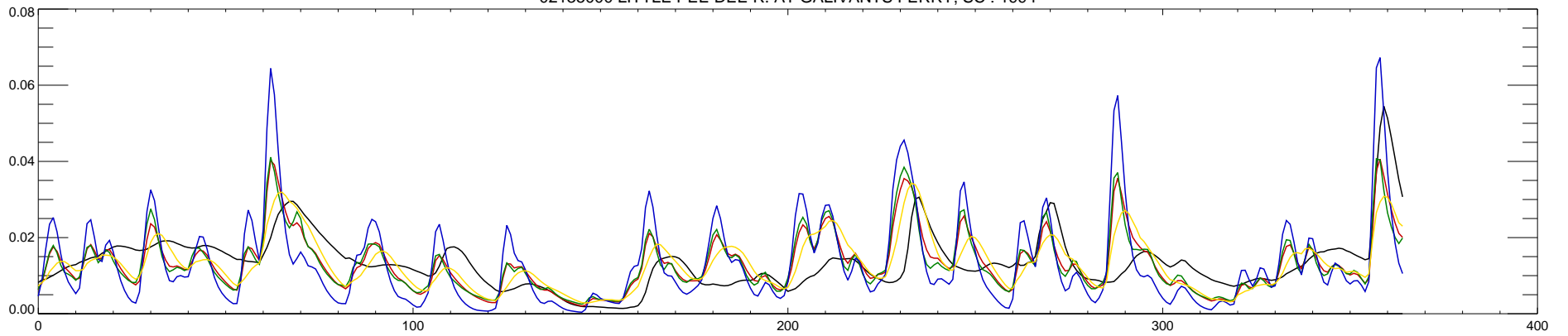
02135000 LITTLE PEE DEE R. AT GALIVANTS FERRY, SC : 1995
