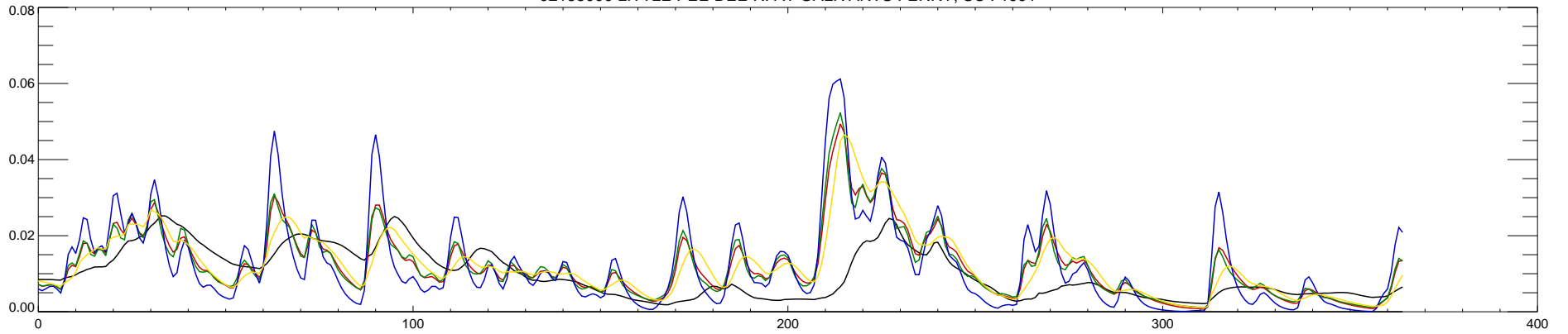
02135000 LITTLE PEE DEE R. AT GALIVANTS FERRY, SC : 1992
