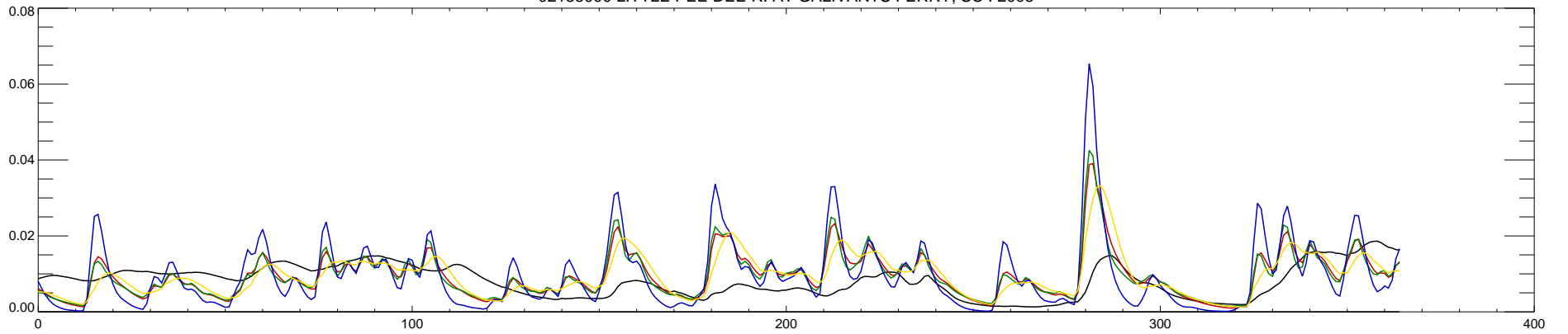
02135000 LITTLE PEE DEE R. AT GALIVANTS FERRY, SC : 2006
