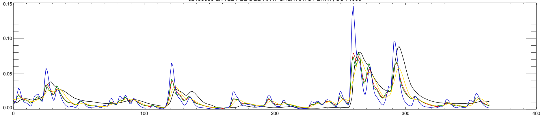
02135000 LITTLE PEE DEE R. AT GALIVANTS FERRY, SC : 2000
