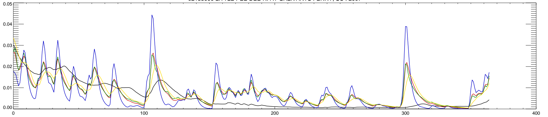
02135000 LITTLE PEE DEE R. AT GALIVANTS FERRY, SC : 2007
