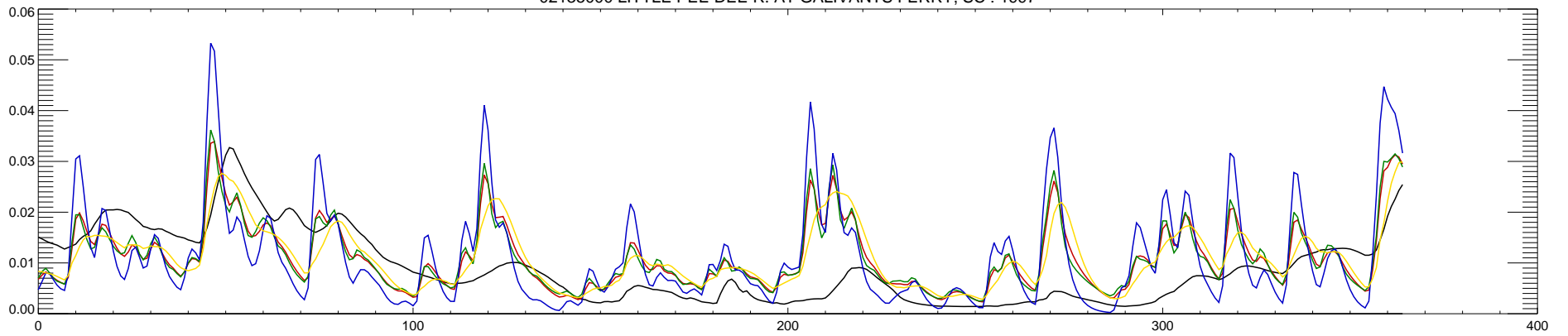
02135000 LITTLE PEE DEE R. AT GALIVANTS FERRY, SC : 1998
