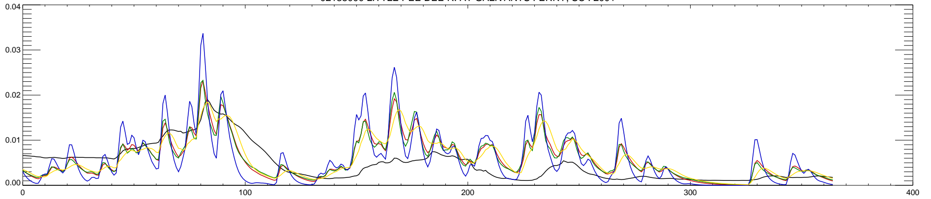
02135000 LITTLE PEE DEE R. AT GALIVANTS FERRY, SC : 2001
