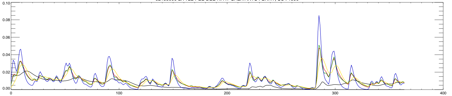
02135000 LITTLE PEE DEE R. AT GALIVANTS FERRY, SC : 1991
