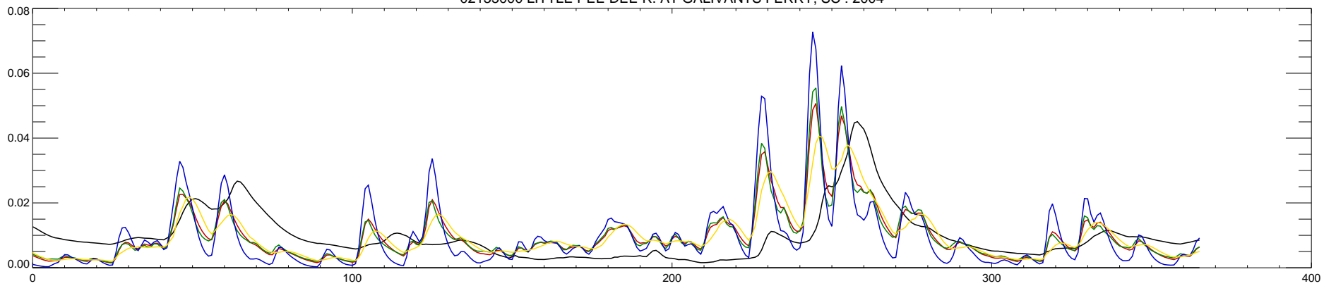
02135000 LITTLE PEE DEE R. AT GALIVANTS FERRY, SC : 2004
