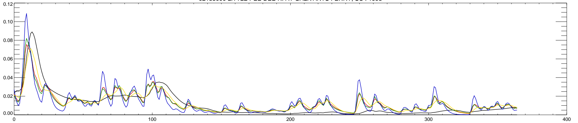
02135000 LITTLE PEE DEE R. AT GALIVANTS FERRY, SC : 1994
