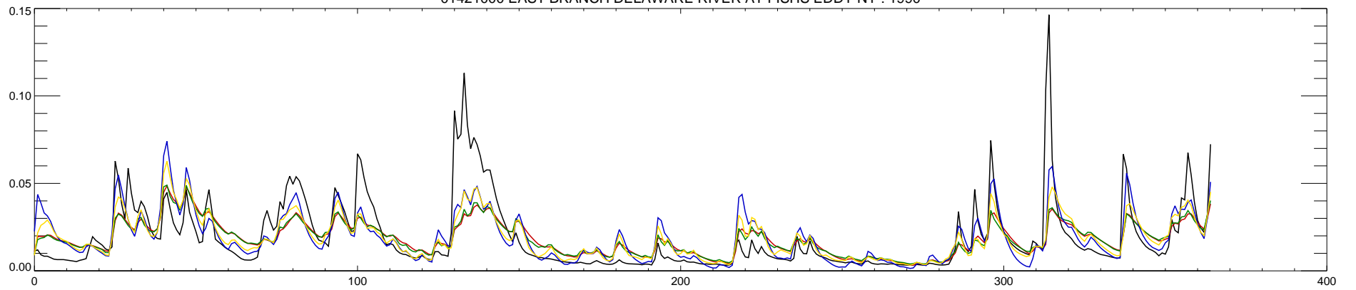
01421000 EAST BRANCH DELAWARE RIVER AT FISHS EDDY NY : 1991
