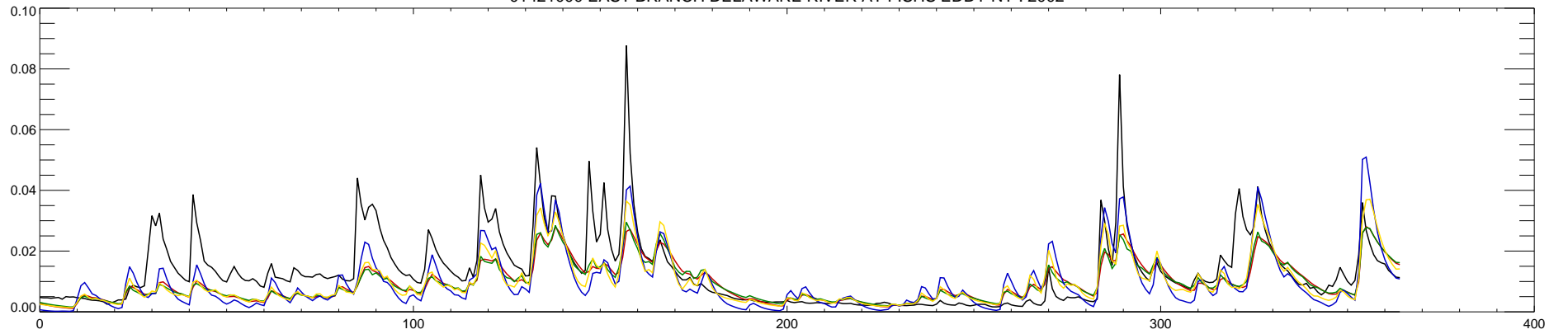
01421000 EAST BRANCH DELAWARE RIVER AT FISHS EDDY NY : 2003
