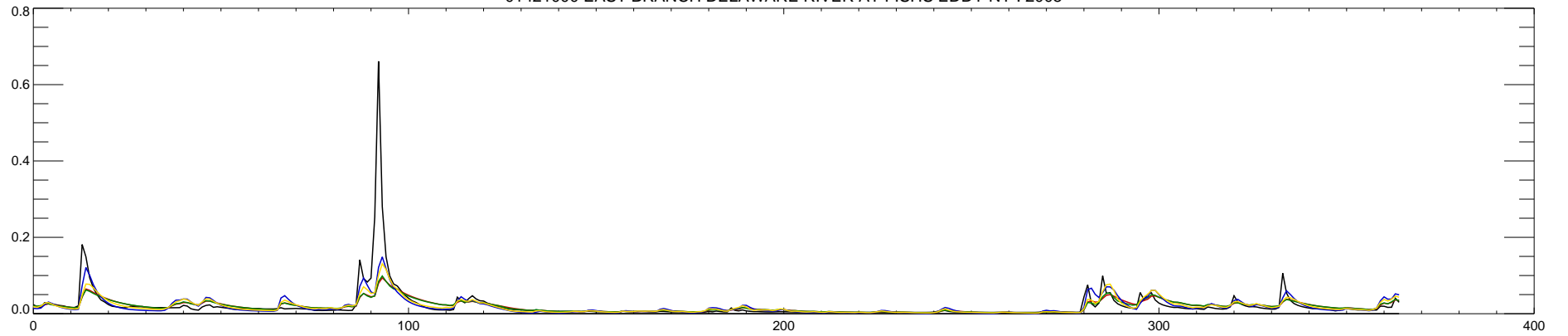
01421000 EAST BRANCH DELAWARE RIVER AT FISHS EDDY NY : 2006
