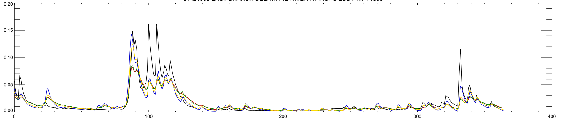
01421000 EAST BRANCH DELAWARE RIVER AT FISHS EDDY NY : 1994
