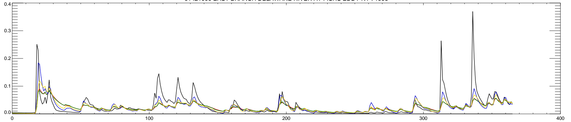
01421000 EAST BRANCH DELAWARE RIVER AT FISHS EDDY NY : 1997
