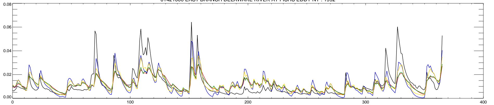
01421000 EAST BRANCH DELAWARE RIVER AT FISHS EDDY NY : 1992
