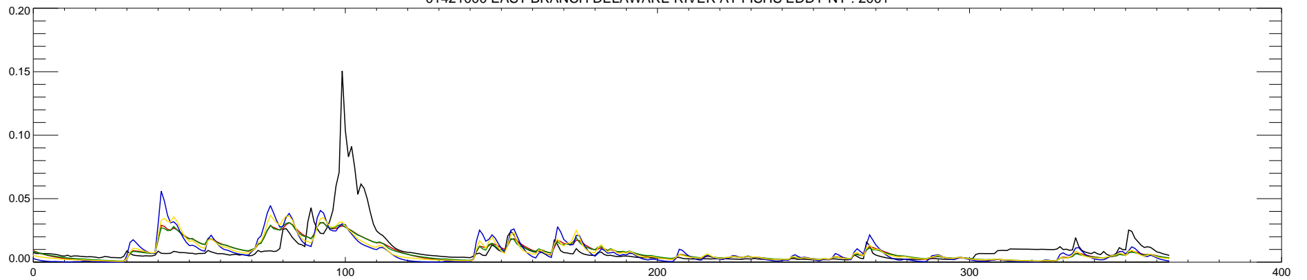
01421000 EAST BRANCH DELAWARE RIVER AT FISHS EDDY NY : 2001
