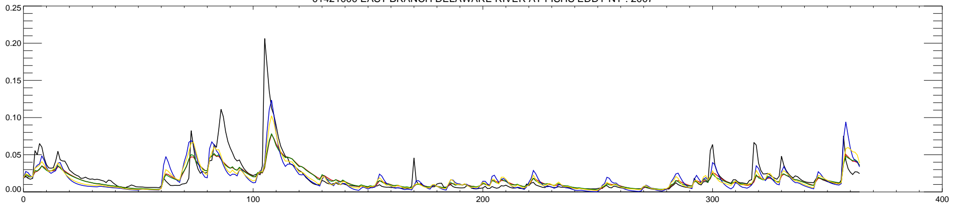
01421000 EAST BRANCH DELAWARE RIVER AT FISHS EDDY NY : 2007
