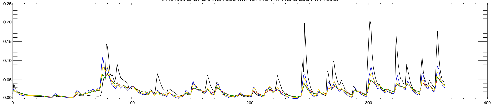
01421000 EAST BRANCH DELAWARE RIVER AT FISHS EDDY NY : 2004
