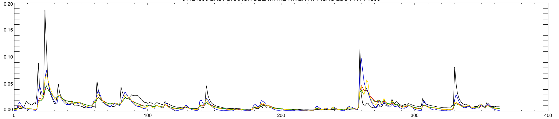
01421000 EAST BRANCH DELAWARE RIVER AT FISHS EDDY NY : 2000
