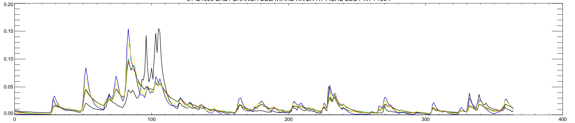
01421000 EAST BRANCH DELAWARE RIVER AT FISHS EDDY NY : 1995
