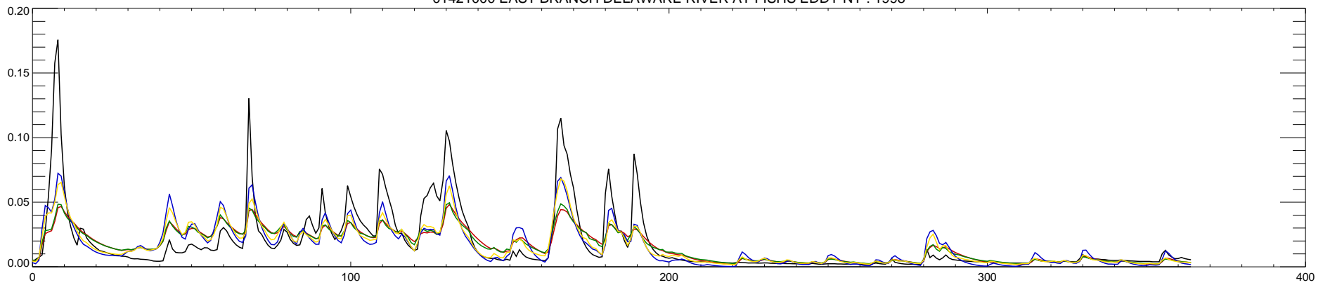
01421000 EAST BRANCH DELAWARE RIVER AT FISHS EDDY NY : 1998
