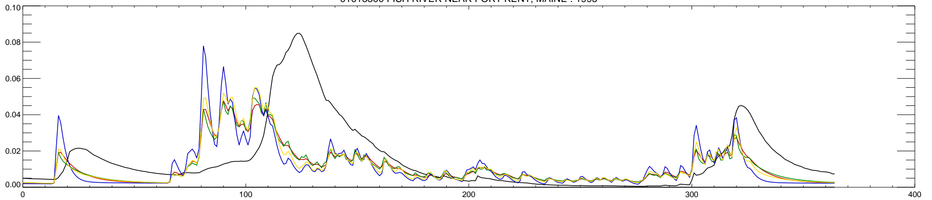
01013500 FISH RIVER NEAR FORT KENT, MAINE : 1995
