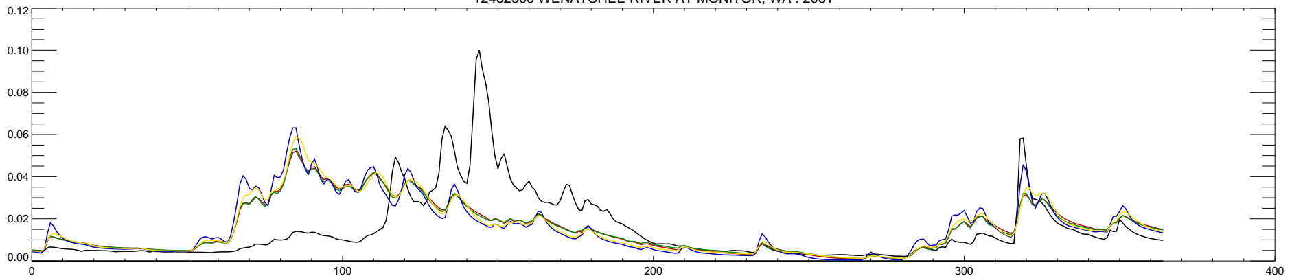
12462500 WENATCHEE RIVER AT MONITOR, WA : 2001
