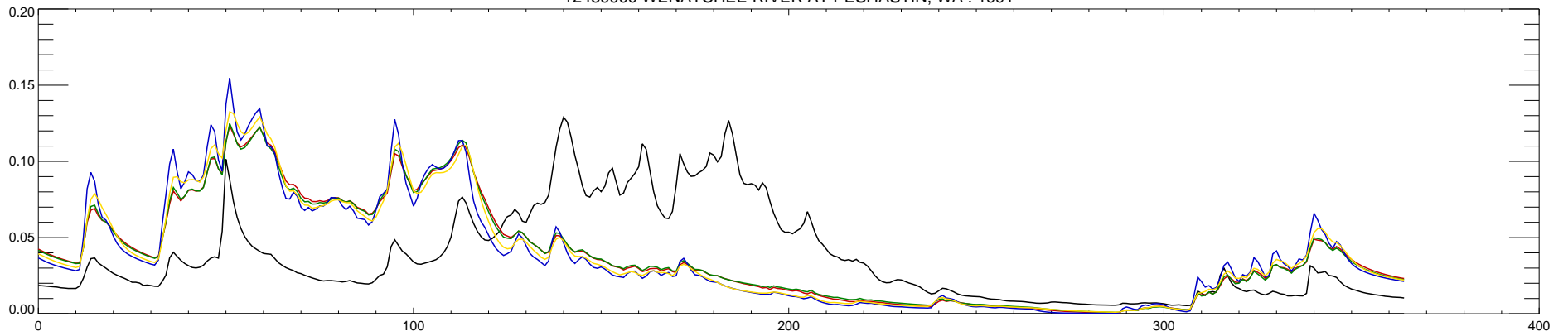
12459000 WENATCHEE RIVER AT PESHASTIN, WA : 1992
