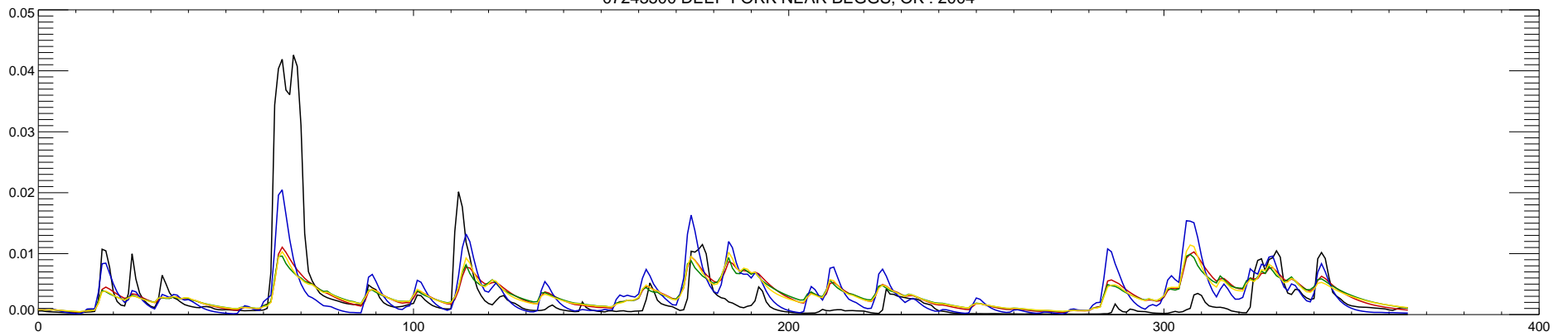
07243500 DEEP FORK NEAR BEGGS, OK : 2004
