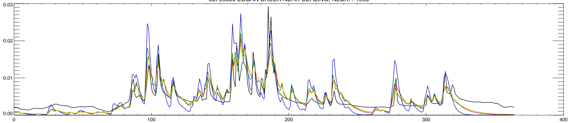
06799500 LOGAN CREEK NEAR UEHLING, NEBR. : 1998
