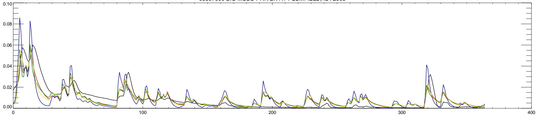
05597000 BIG MUDDY RIVER AT PLUMFIELD, IL : 2006
