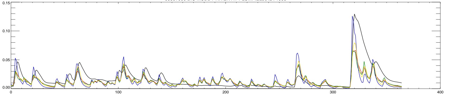
05597000 BIG MUDDY RIVER AT PLUMFIELD, IL : 1994
