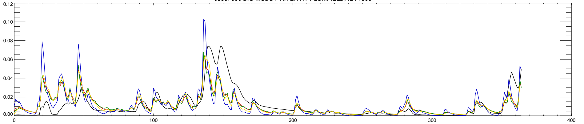
05597000 BIG MUDDY RIVER AT PLUMFIELD, IL : 1991
