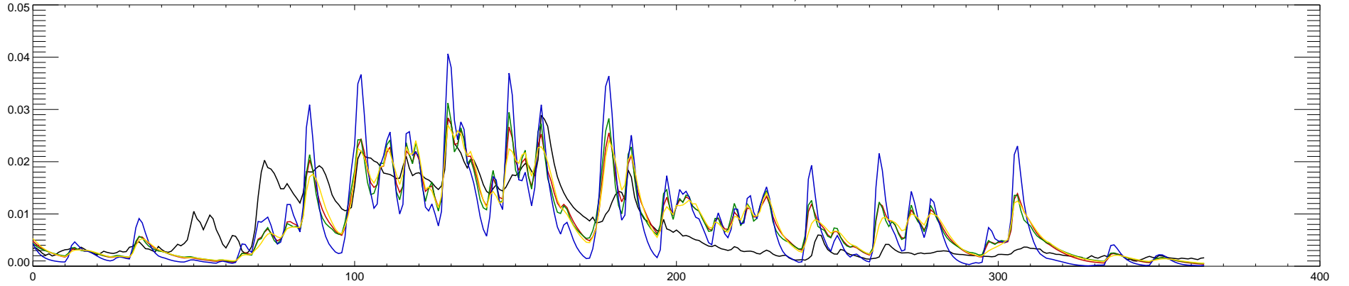
05451500 IOWA RIVER AT MARSHALLTOWN, IA : 1995
