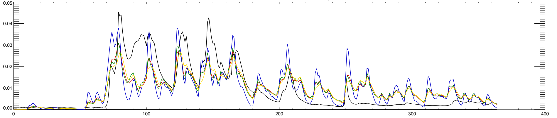
05451500 IOWA RIVER AT MARSHALLTOWN, IA : 2001
