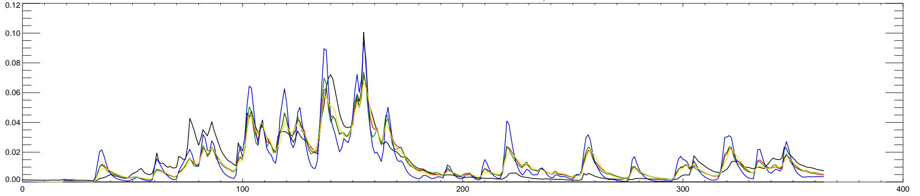
05451500 IOWA RIVER AT MARSHALLTOWN, IA : 1992
