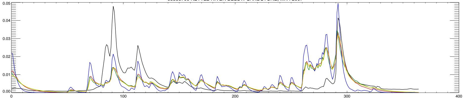
05336700 KETTLE RIVER BELOW SANDSTONE, MN : 2007
