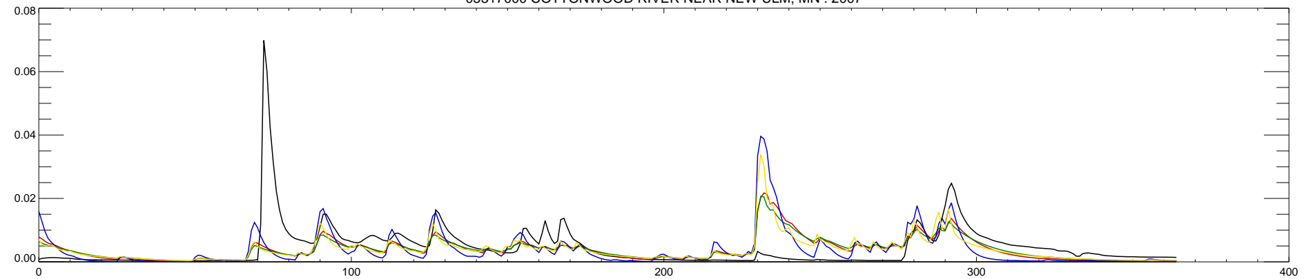
05317000 COTTONWOOD RIVER NEAR NEW ULM, MN : 2007
