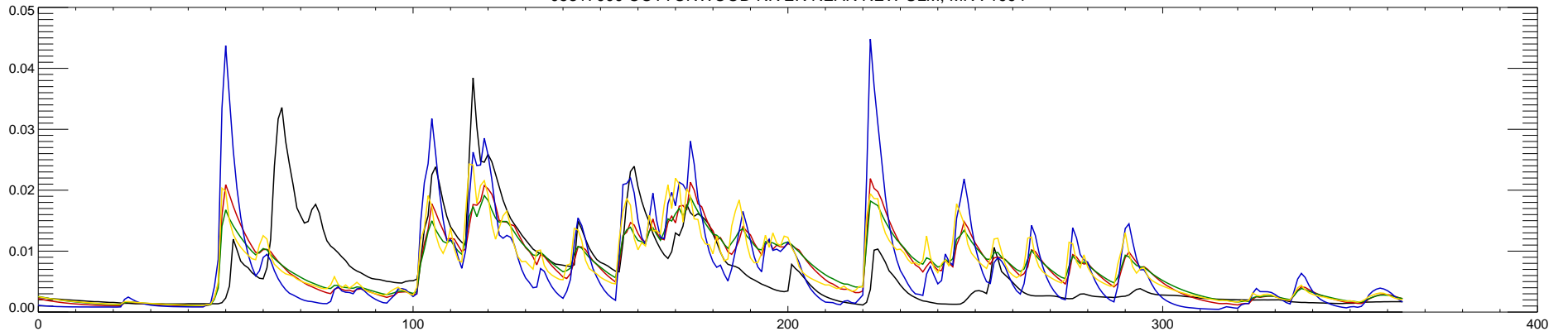
05317000 COTTONWOOD RIVER NEAR NEW ULM, MN : 1995
