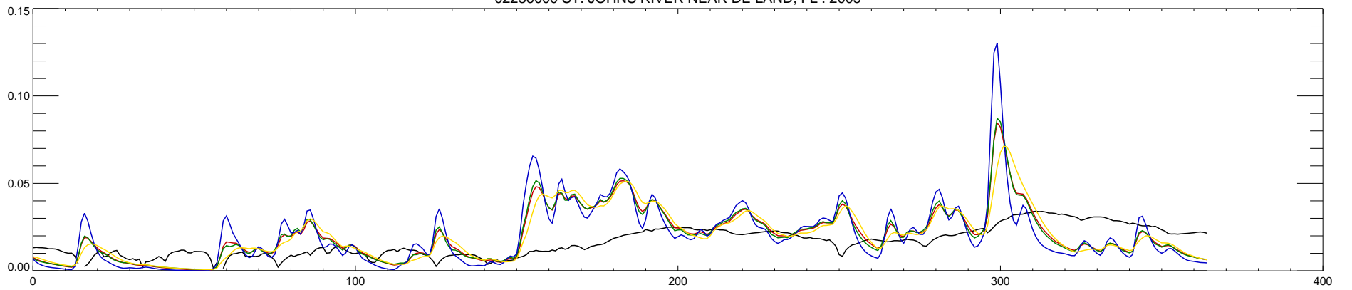
02236000 ST. JOHNS RIVER NEAR DE LAND, FL : 2006
