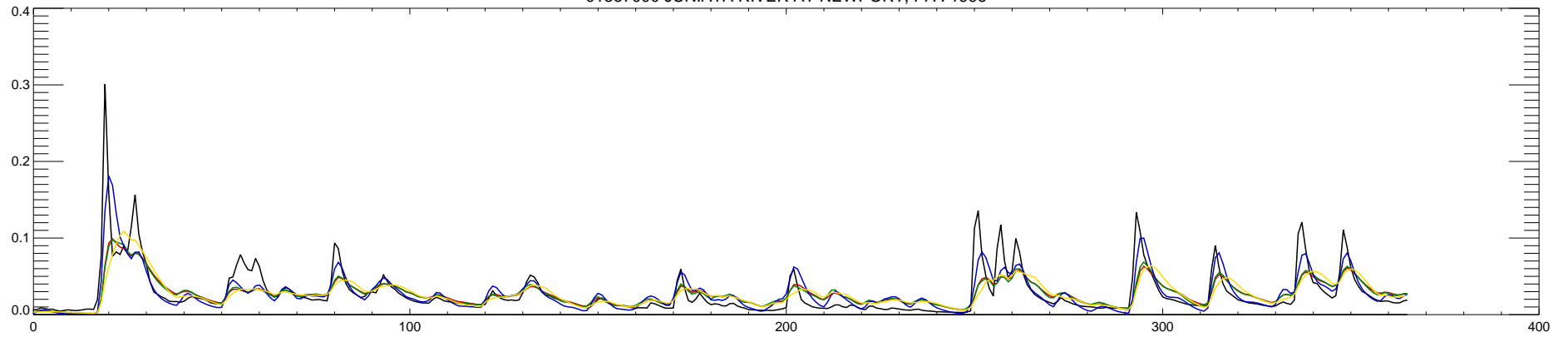
01567000 JUNIATA RIVER AT NEWPORT, PA : 1997
