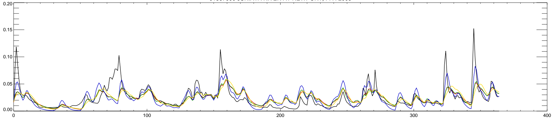
01567000 JUNIATA RIVER AT NEWPORT, PA : 2004
