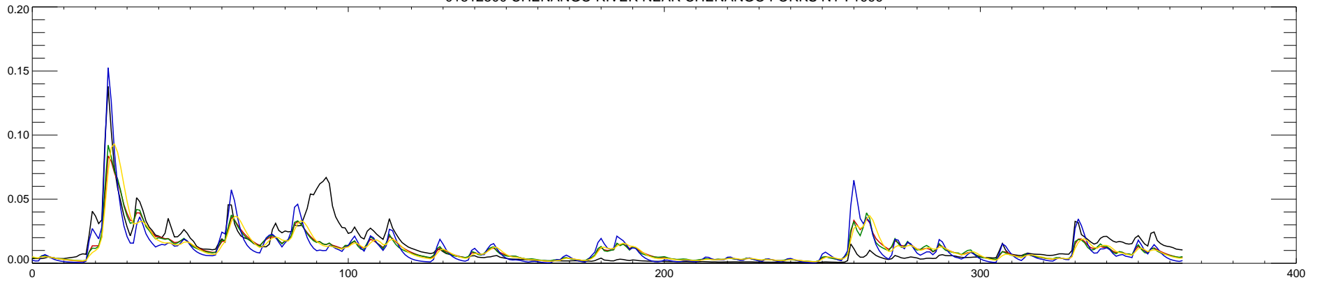
01512500 CHENANGO RIVER NEAR CHENANGO FORKS NY : 2000
