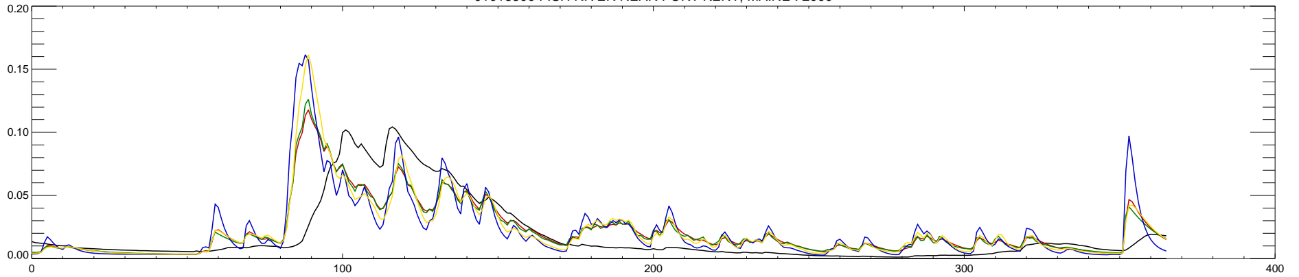
01013500 FISH RIVER NEAR FORT KENT, MAINE : 2001
