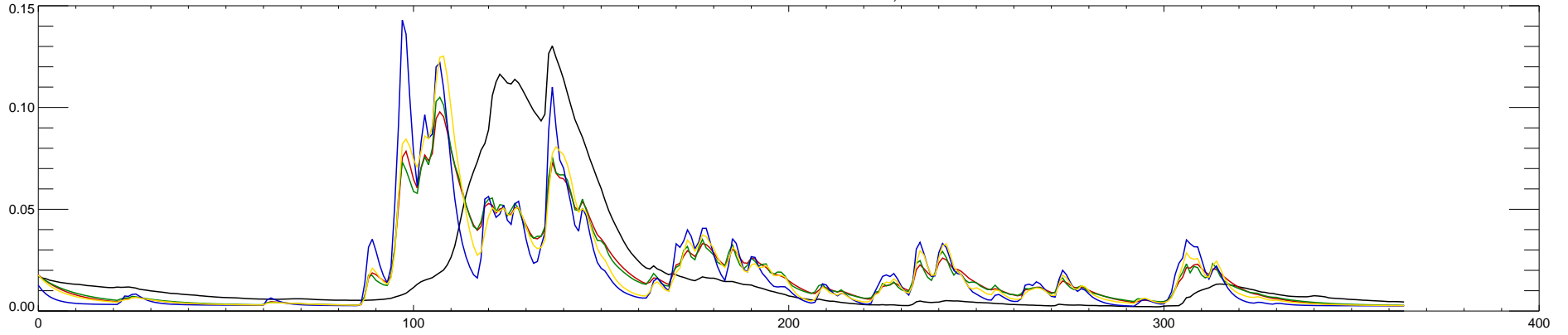
01013500 FISH RIVER NEAR FORT KENT, MAINE : 1998
