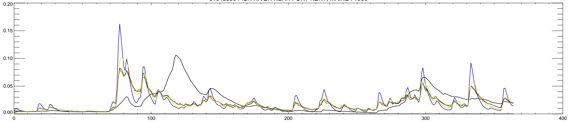
01013500 FISH RIVER NEAR FORT KENT, MAINE : 1991
