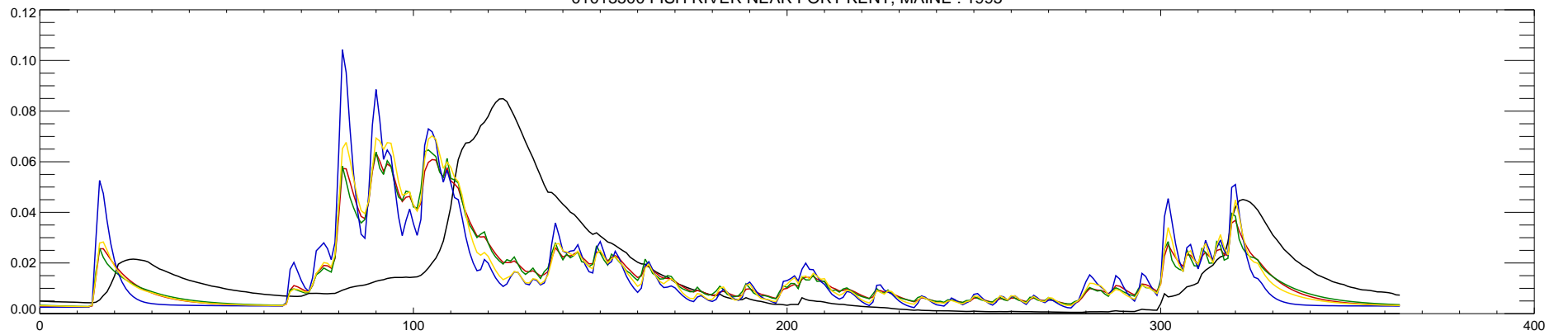
01013500 FISH RIVER NEAR FORT KENT, MAINE : 1995
