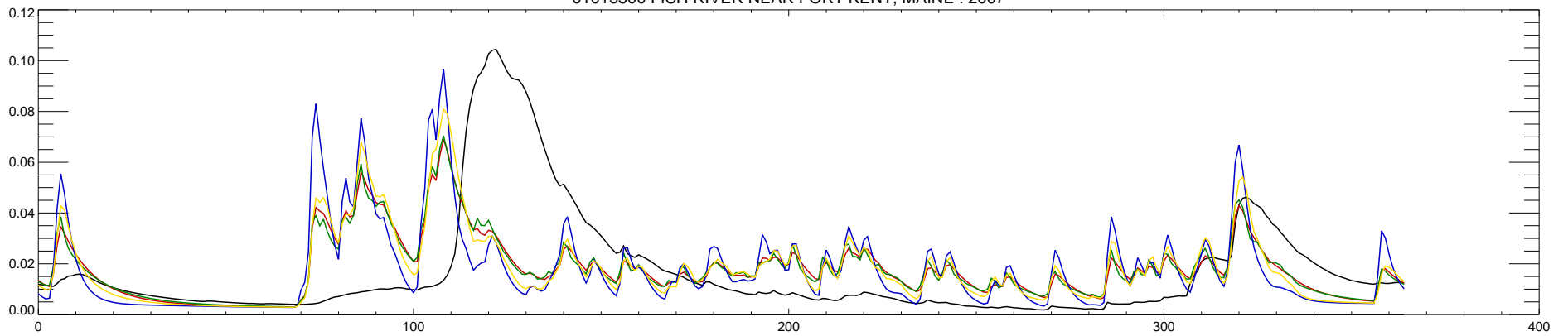
01013500 FISH RIVER NEAR FORT KENT, MAINE : 2007
