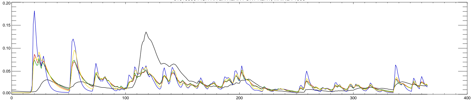
01013500 FISH RIVER NEAR FORT KENT, MAINE : 1997
