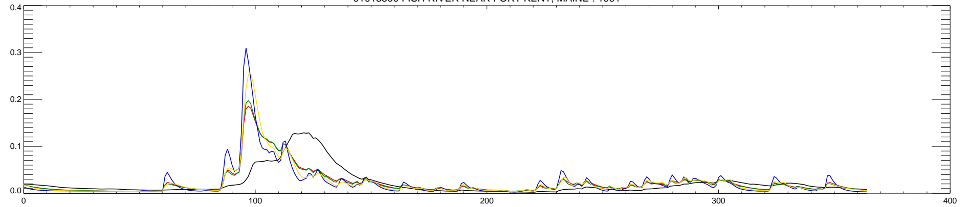
01013500 FISH RIVER NEAR FORT KENT, MAINE : 1992
