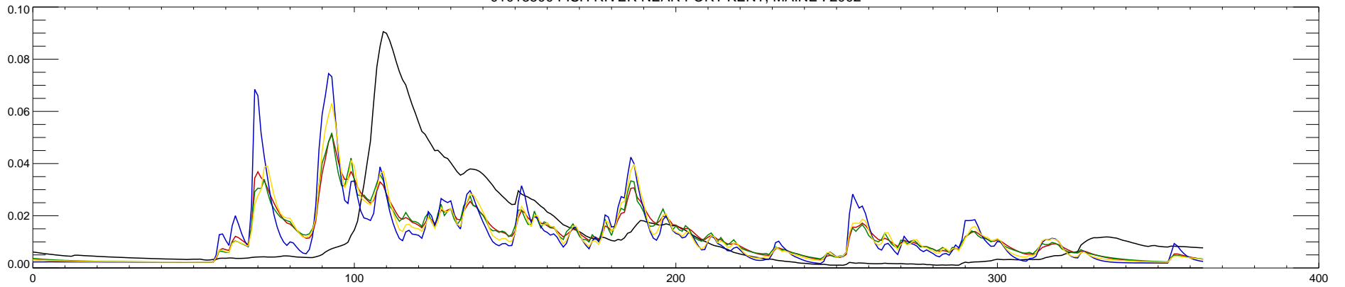
01013500 FISH RIVER NEAR FORT KENT, MAINE : 2003
