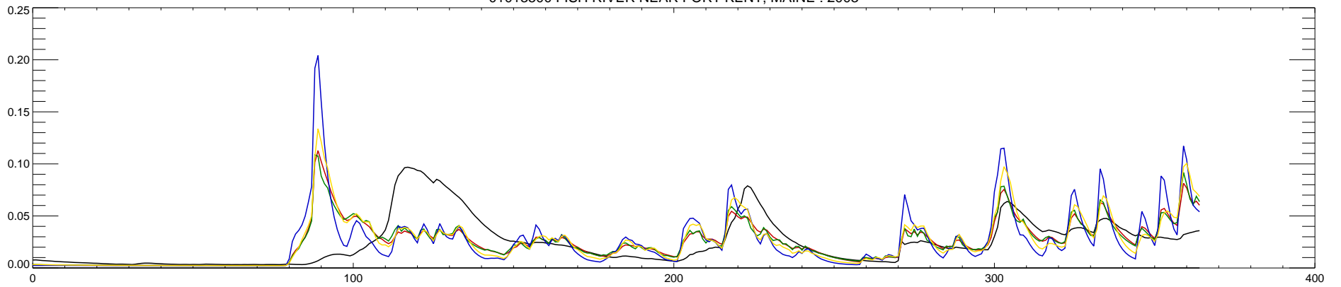
01013500 FISH RIVER NEAR FORT KENT, MAINE : 2004
