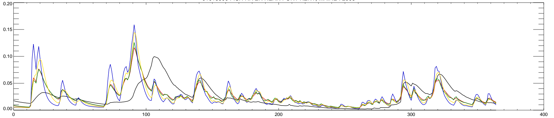
01013500 FISH RIVER NEAR FORT KENT, MAINE : 2007
