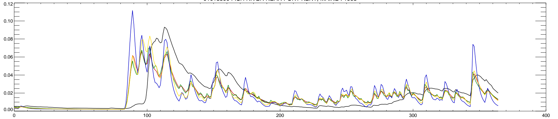
01013500 FISH RIVER NEAR FORT KENT, MAINE : 1994
