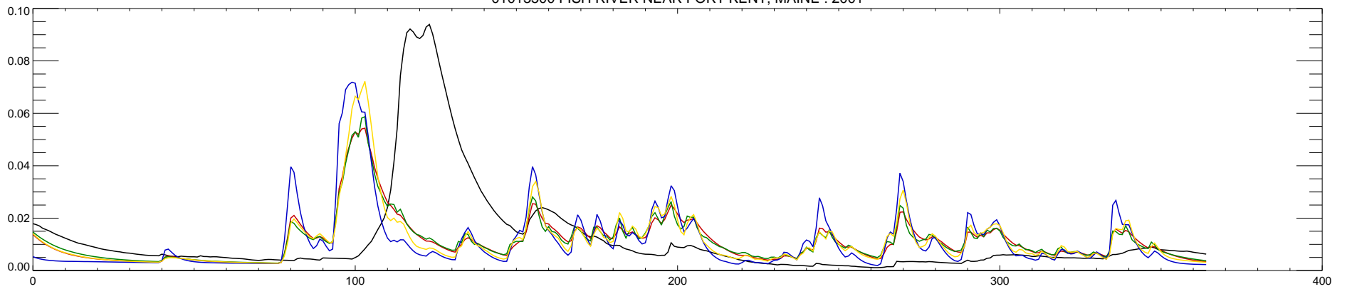
01013500 FISH RIVER NEAR FORT KENT, MAINE : 2001
