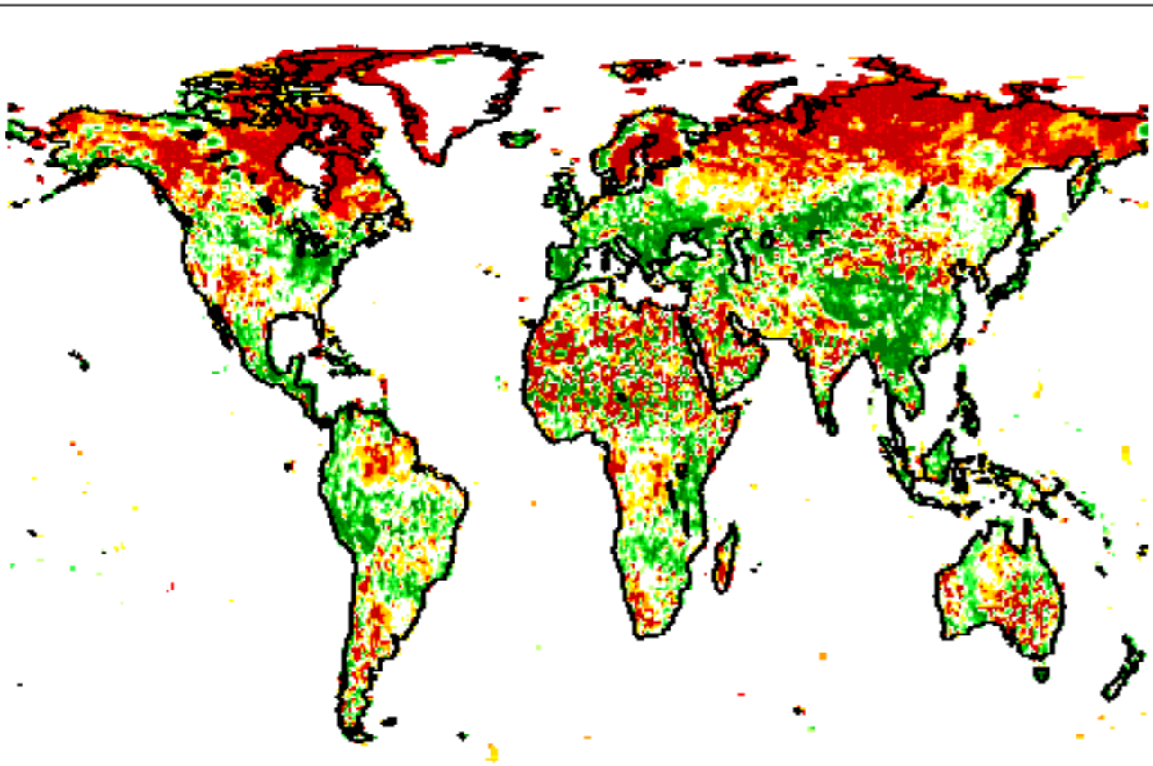
Initial Conditions: 27 Mar 2018
