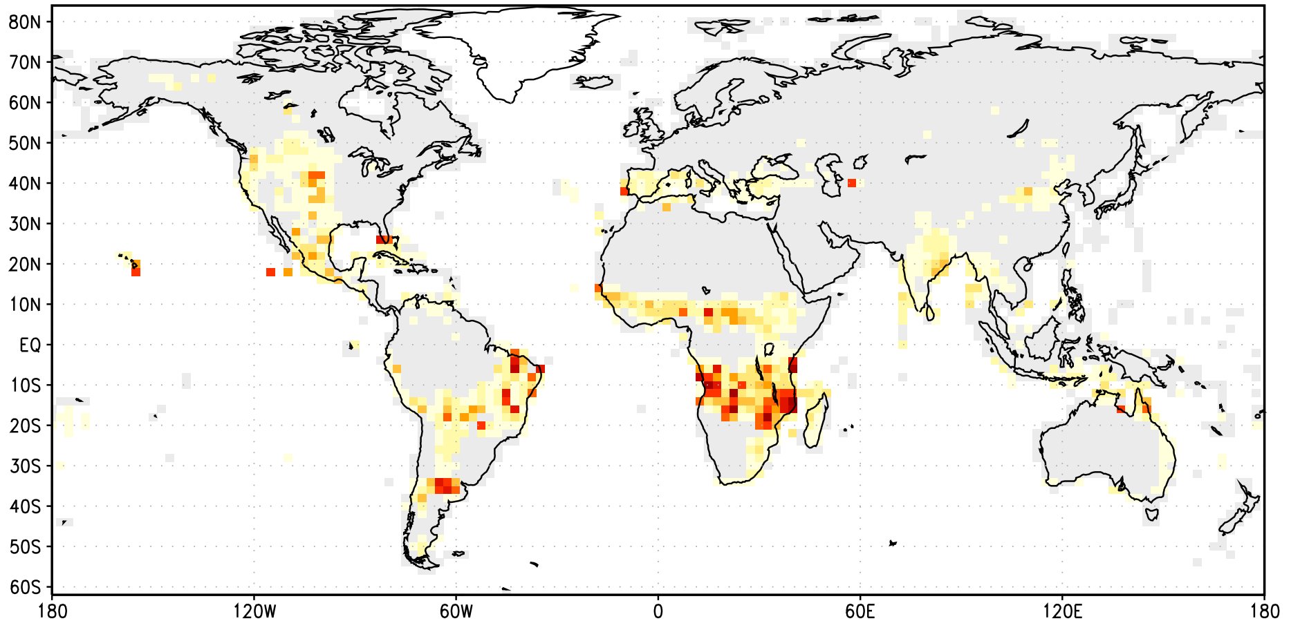
Annual mean burn area (%/yr), p0007s–p0006s, ens=35
