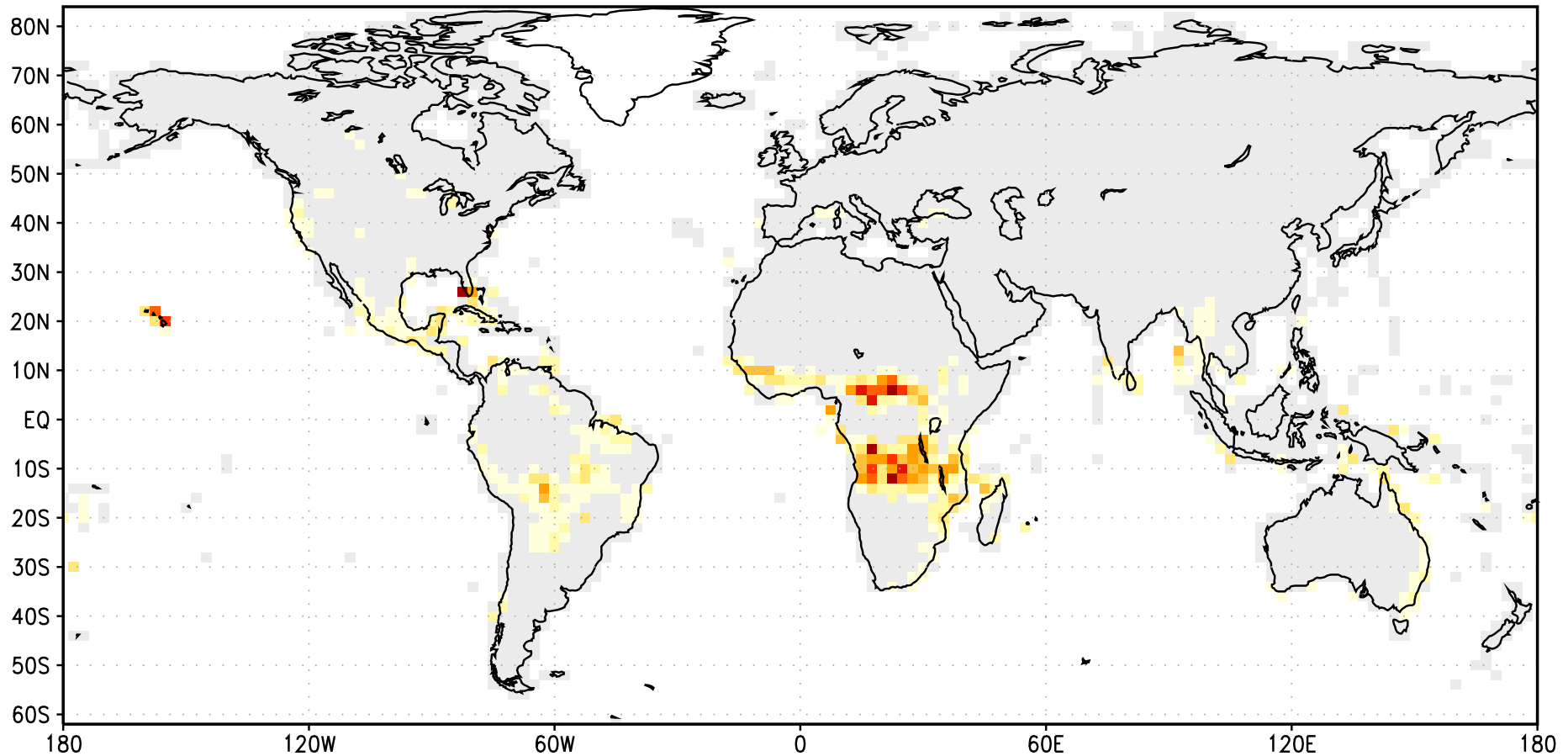
Annual carbon loss (gC/m 2 /yr), p0007s–p0006s, ens=35
