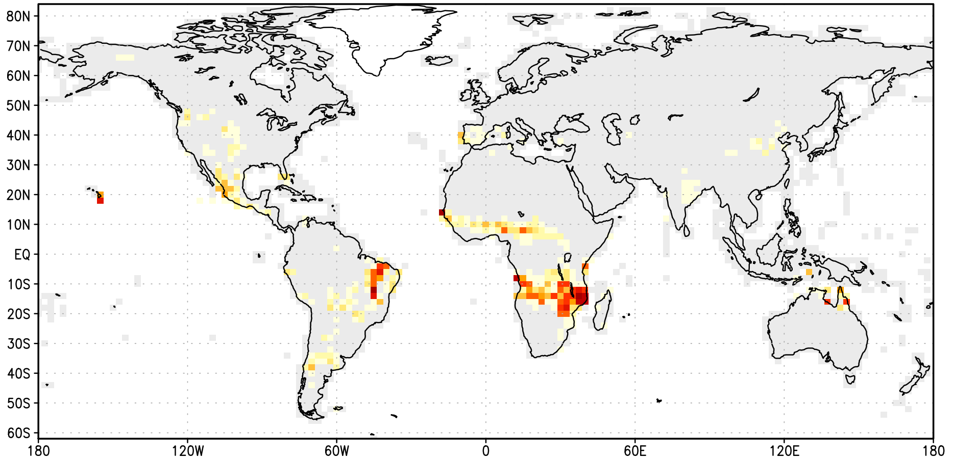
Annual mean burn area (%/yr), p0006s, ens=35
