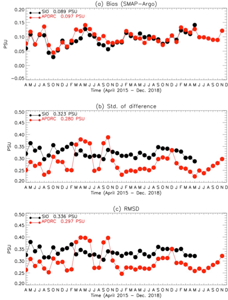
Figure 4.2: Monthly (a) mean difference (SMAP minus Argo), (b) the standard deviation and (c) RMS difference between SMAP V4.2 and the gridded Argo product from SIO (black) and APDRC (red).
