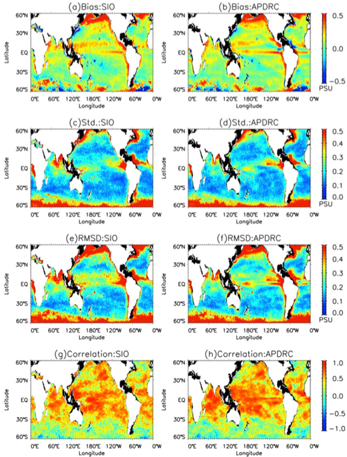
Figure 4.1: Comparison of SMAP SSS V4.2 with the monthly gridded Argo product from SIO (left) and APDRC (right): (a & b) Biases, (c & d) standard deviation, (e & f) RMS difference and (g & h) correlation coefficients for the period from April 2015 to November 2018.
