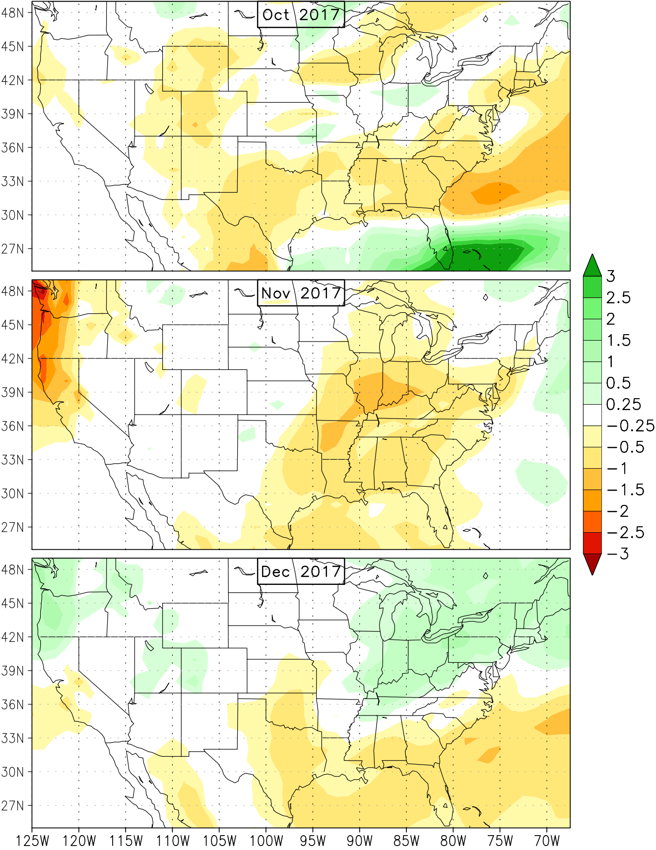
stats from 36 year climatology
